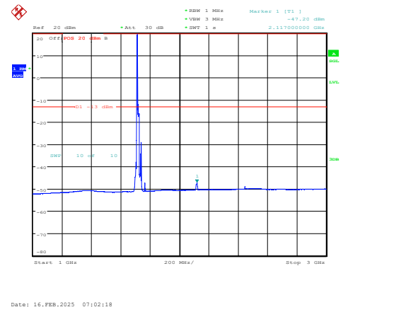
Band4-15MHz-QPSK-20025-1RB#0-1000~3000-P ASS
