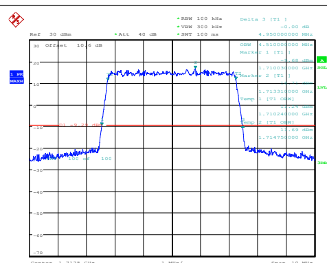
Band4-5MHz-QPSK-19975-25RB#0-PASS
