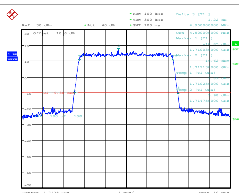
Band4-5MHz-16QAM-19975-25RB#0-PASS
