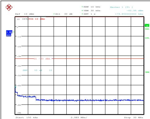
Band4-1.4MHz-16QAM-20175-1RB#0-0.15~30-P ASS
