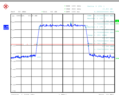
Band4-5MHz-QPSK-19975-25RB#0-PASS
