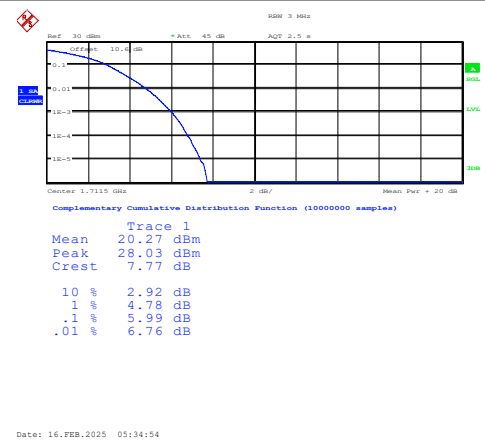
Band4-3MHz-16QAM-19965-15RB#0-PASS
