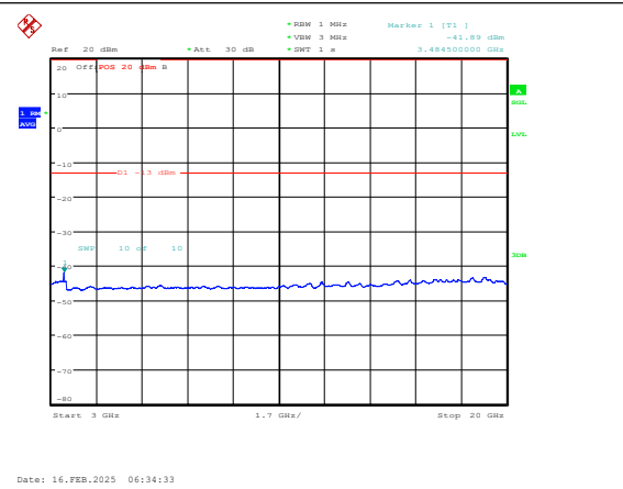
Band4-10MHz-16QAM-20350-1RB#0-3000~20000 -PASS
