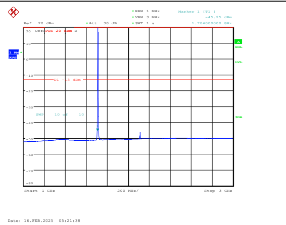
Band4-3MHz-QPSK-19965-1RB#0-1000~3000-PASS S
