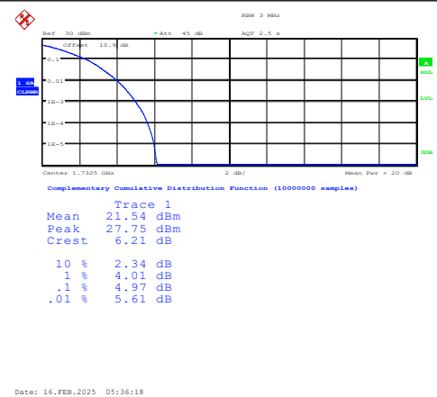
Band4-3MHz-QPSK-20175-15RB#0-PASS
