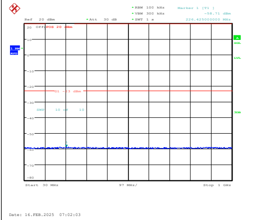
Band4-15MHz-QPSK-20025-1RB#0-30~1000-PA SS
