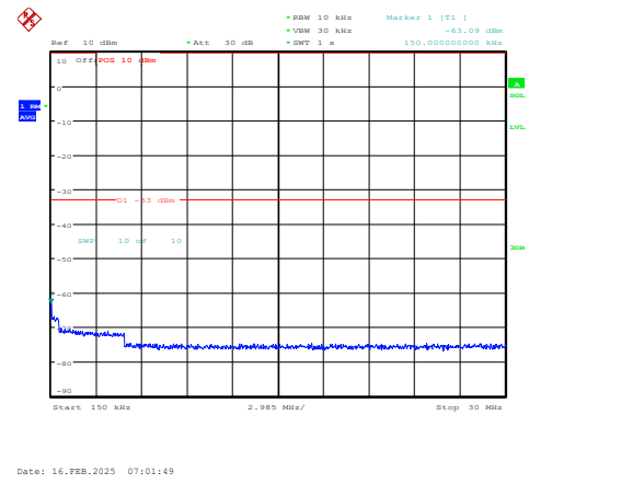
Band4-15MHz-QPSK-20025-1RB#0-0.15~30-PAS S
