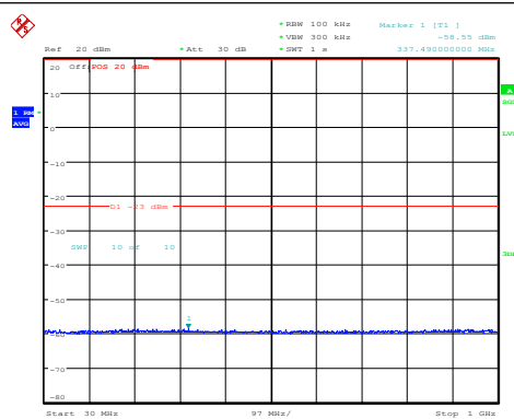
Band4-5MHz-16QAM-20175-1RB#0-30~1000-PAS S
