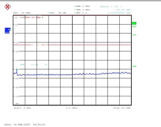
Band4-1.4MHz-16QAM-20393-1RB#0-3000~2000 0-PASS
