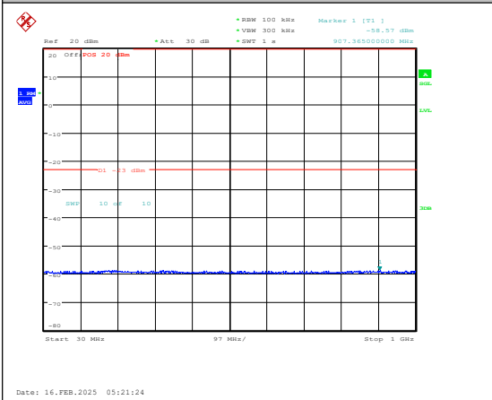
Band4-3MHz-QPSK-19965-1RB#0-30~1000-PAS S
