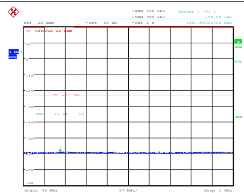
Band4-1.4MHz-16QAM-20175-1RB#0-30~1000-P ASS
