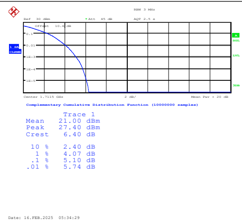
Band4-3MHz-QPSK-19965-15RB#0-PASS
