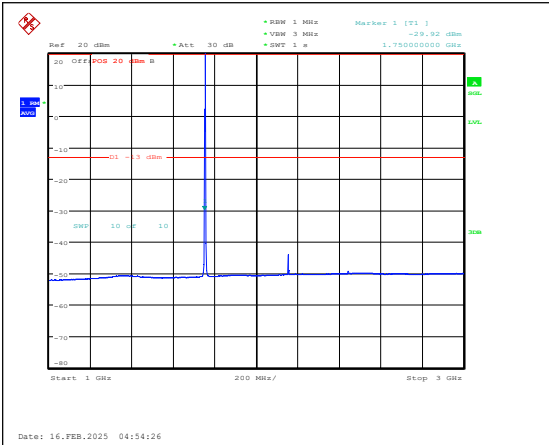
Band4-1.4MHz-16QAM-20393-1RB#0-1000~300 0-PASS
