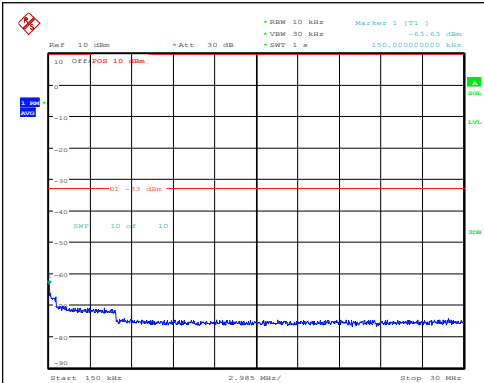
Band4-5MHz-16QAM-20175-1RB#0-0.15~30-PA SS
