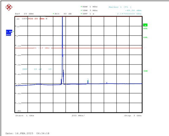
Band4-10MHz-16QAM-20350-1RB#0-1000~3000 -PASS
