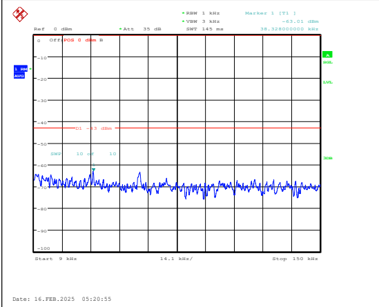
Band4-3MHz-QPSK-19965-1RB#0-0.009~0.15-P ASS
