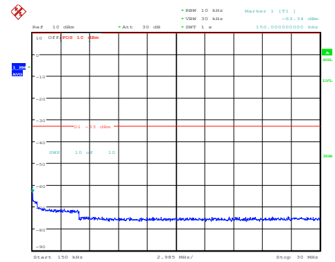
Band4-1.4MHz-16QAM-20175-1RB#0-3000~2000 0-PASS
