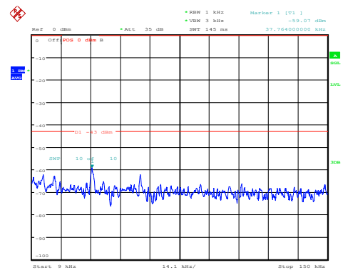
Band2-5MHz-QPSK-18900-1RB#0-1000~3000-PA SS
