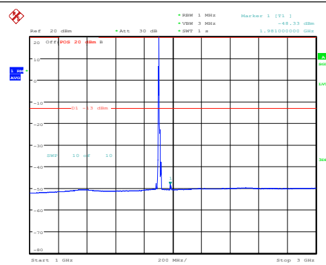
Band2-10MHz-QPSK-19150-1RB#0-1000~3000-P ASS
