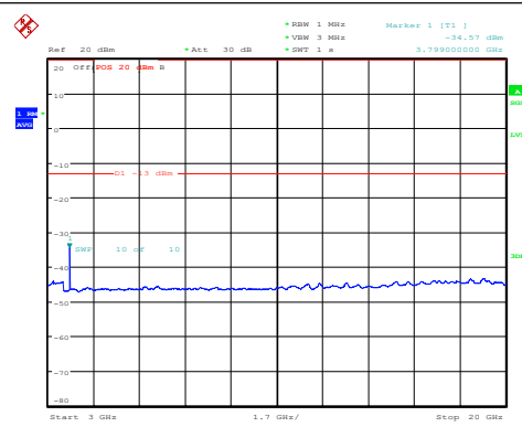
Band2-10MHz-16QAM-19150-1RB#0-3000~20000 -PASS
