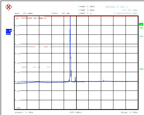
Band2-10MHz-16QAM-19150-1RB#0-1000~3000 -PASS
