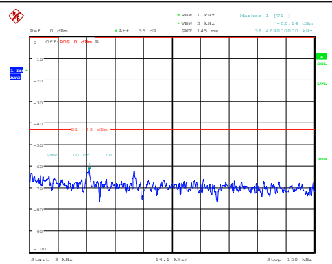
Band2-5MHz-16QAM-18625-1RB#0-0.009~0.15-P ASS
