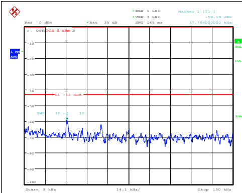
Band2-5MHz-QPSK-18900-1RB#0-0.009~0.15-P ASS
