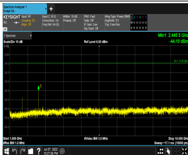
Band26-15MHz-QPSK-26765-1RB#0-Range3:1000~10000MHz
