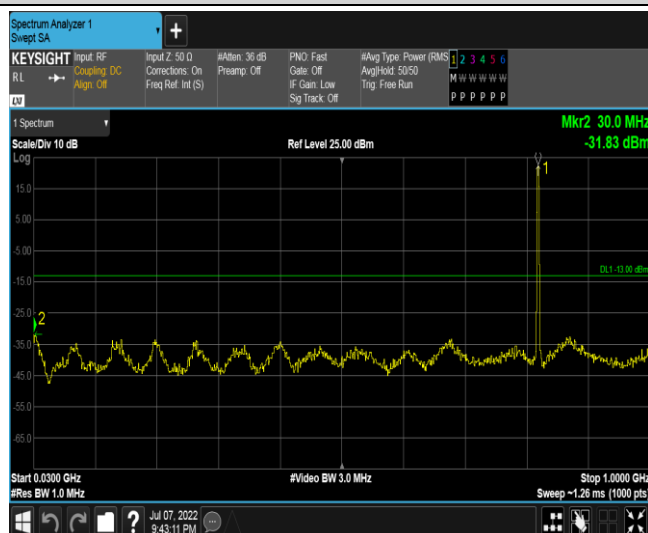
Band26-1.4MHz-QPSK-26783-1RB#0-Range2:30~1000MHz
