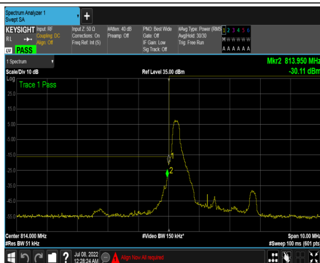
Band26-3MHz-QPSK-26705-1RB#14
