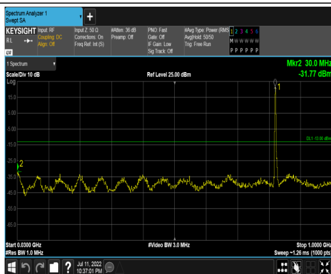
Band26-5MHz-QPSK-26815-1RB#0-Range2:30~1000MHz
