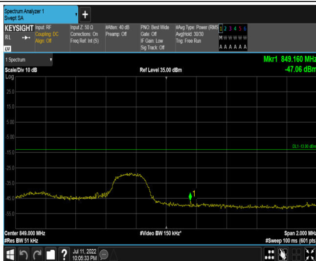
Band26-3MHz-QPSK-27025-1RB#14
