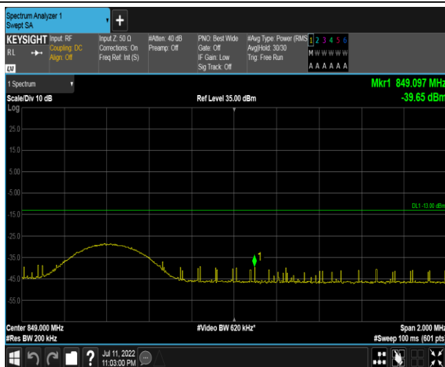
Band26-10MHz-16QAM-26990-1RB#49
