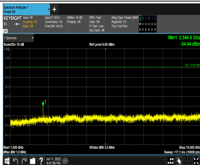
Band26-1.4MHz-QPSK-27033-1RB#0-Range3:1000~10000MHz
