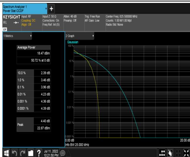
Band26-3MHz-QPSK-26805-1RB#0
