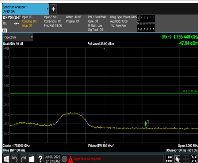
Band4-5MHz-QPSK-20375-1RB#24
