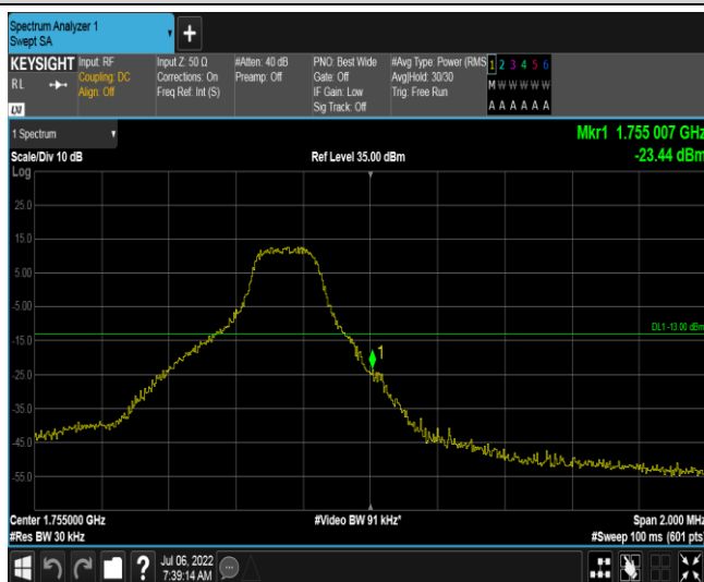
Band4-1.4MHz-QPSK-20393-1RB#5
