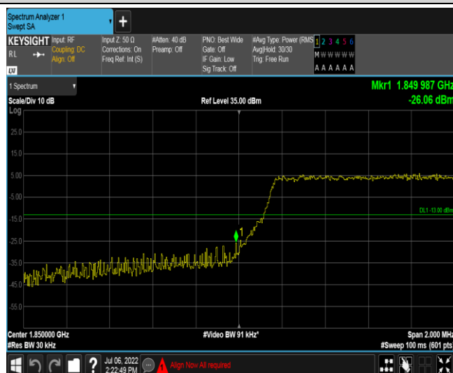
Band25-1.4MHz-16QAM-26683-1RB#0
