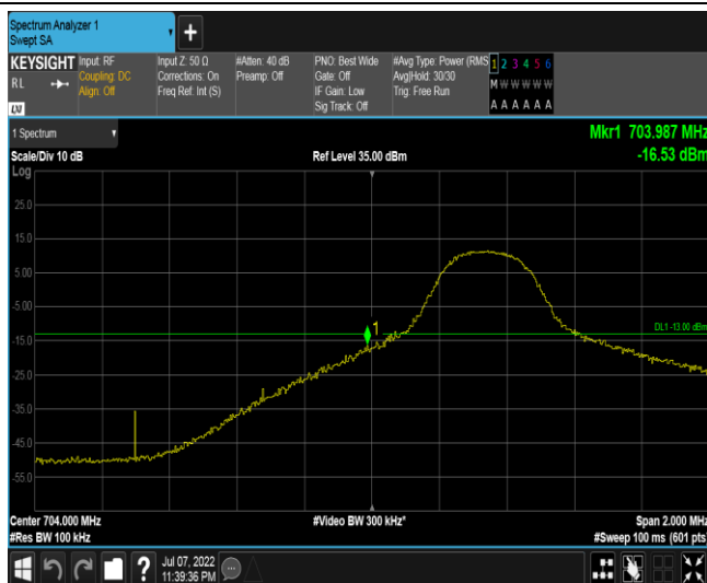
Band17-5MHz-QPSK-23755-1RB#24
