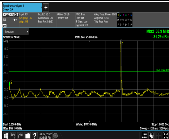
Band17-5MHz-QPSK-23755-1RB#0-Range1:30~1000MHz
