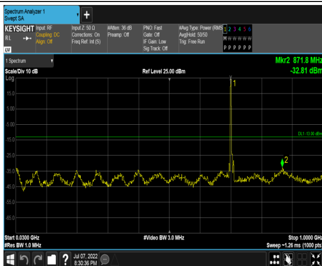
Band17-5MHz-16QAM-23790-1RB#0-Range2:30~1000MHz
