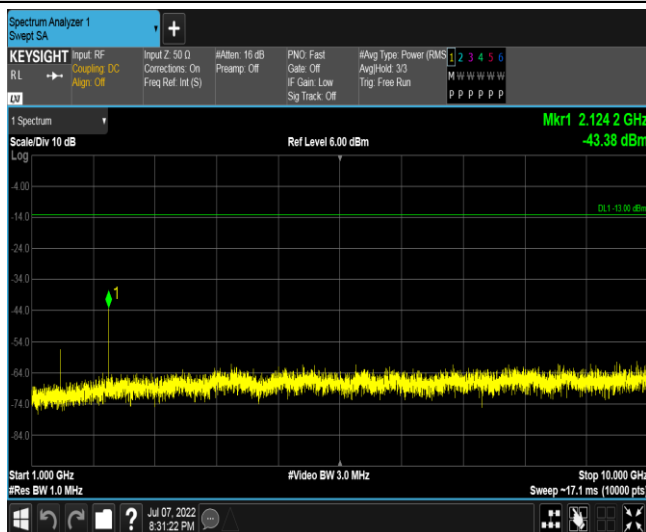
Band17-5MHz-16QAM-23790-1RB#0-Range3:1000~10000MHz
