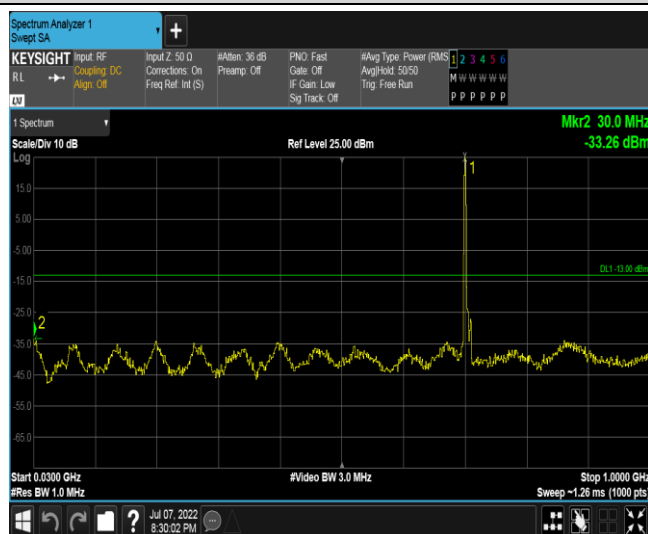
Band17-5MHz-QPSK-23790-1RB#0-Range2:30~1000MHz
