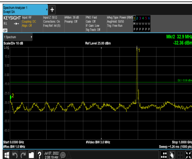
Band12-10MHz-QPSK-23095-1RB#0-Range2:30~1000MHz
