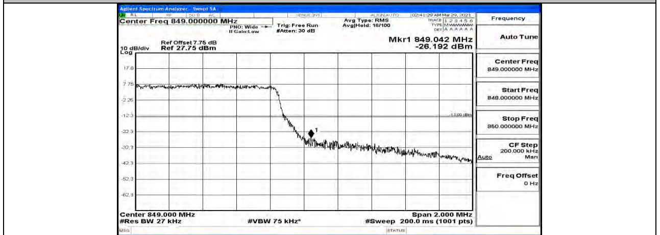
Band Edge Test Graph(s) (Channel Bandwidth: 1.4 MHz)_HCH_16QAM
