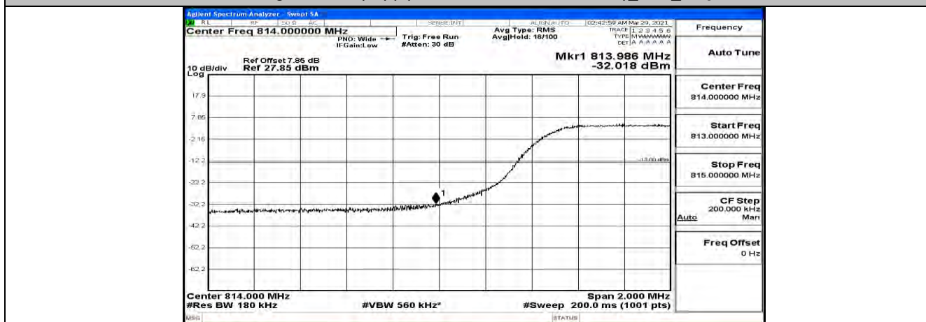
Band Edge Test Graph(s) (Channel Bandwidth: 10 MHz)_LCH_16QAM
