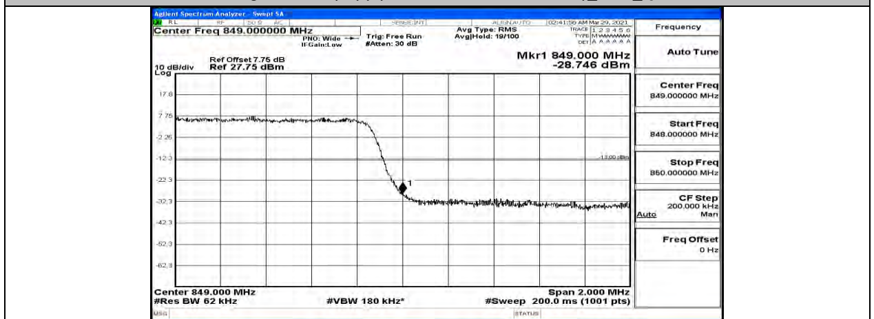
Band Edge Test Graph(s) (Channel Bandwidth: 3 MHz)_HCH_QPSK
