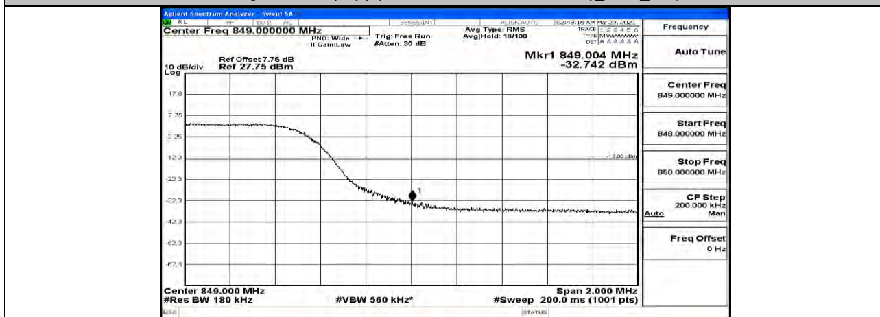
Band Edge Test Graph(s) (Channel Bandwidth: 10 MHz)_HCH_16QAM
