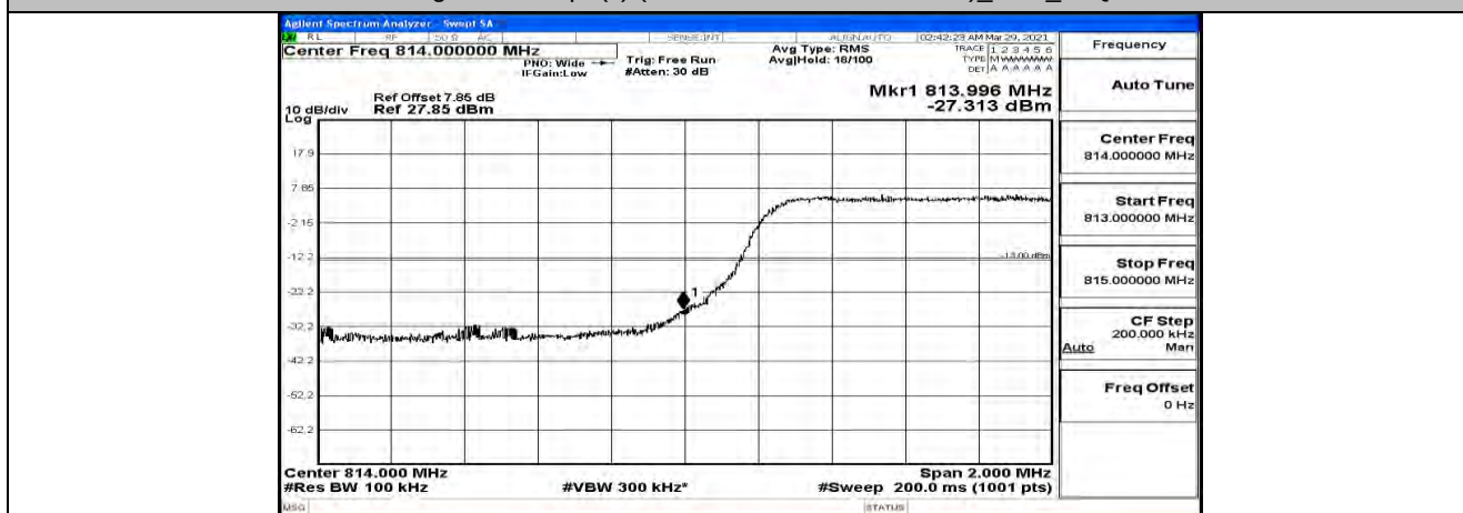
Band Edge Test Graph(s) (Channel Bandwidth: 5 MHz)_LCH_16QAM
