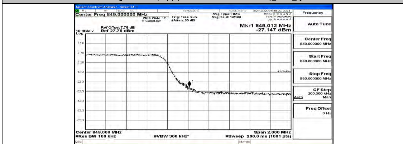
Band Edge Test Graph(s) (Channel Bandwidth: 5 MHz)_HCH_QPSK
