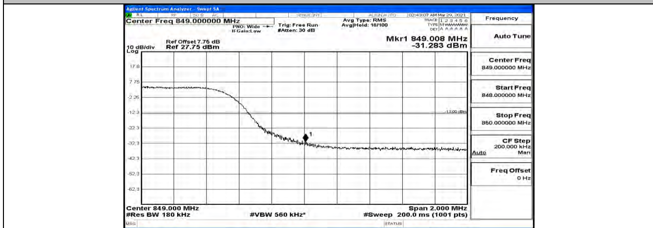
Band Edge Test Graph(s) (Channel Bandwidth: 10 MHz)_HCH_QPSK
