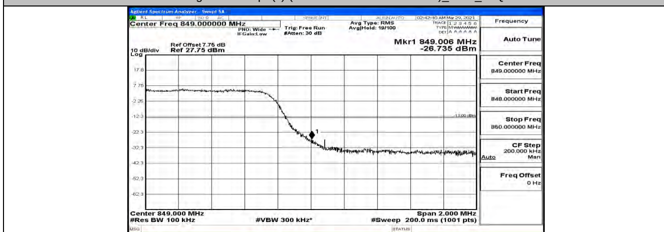
Band Edge Test Graph(s) (Channel Bandwidth: 5 MHz)_HCH_16QAM
