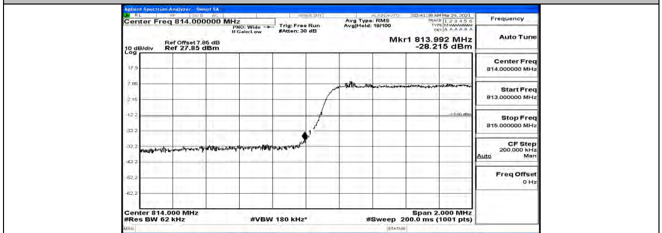
Band Edge Test Graph(s) (Channel Bandwidth: 3 MHz)_LCH_QPSK
