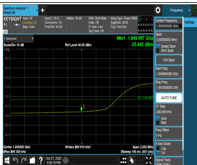
Band2-15MHz-16QAM-19125-1RB#0
