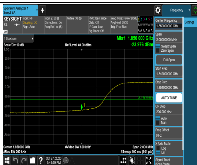
Band2-10MHz-QPSK-19150-1RB#0
