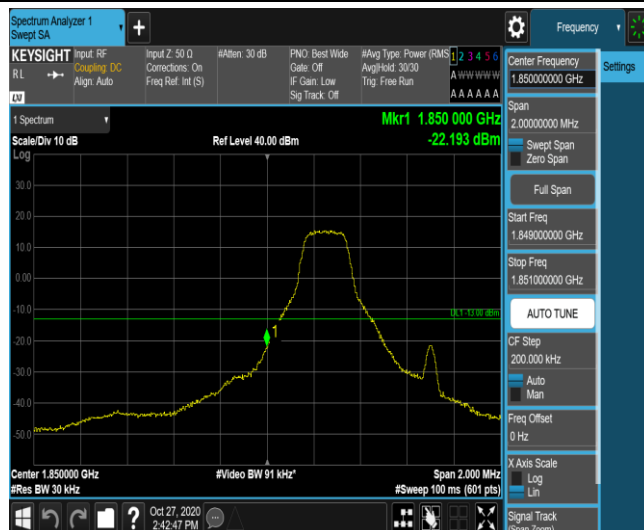
Band2-1.4MHz-QPSK-18607-1RB#5
