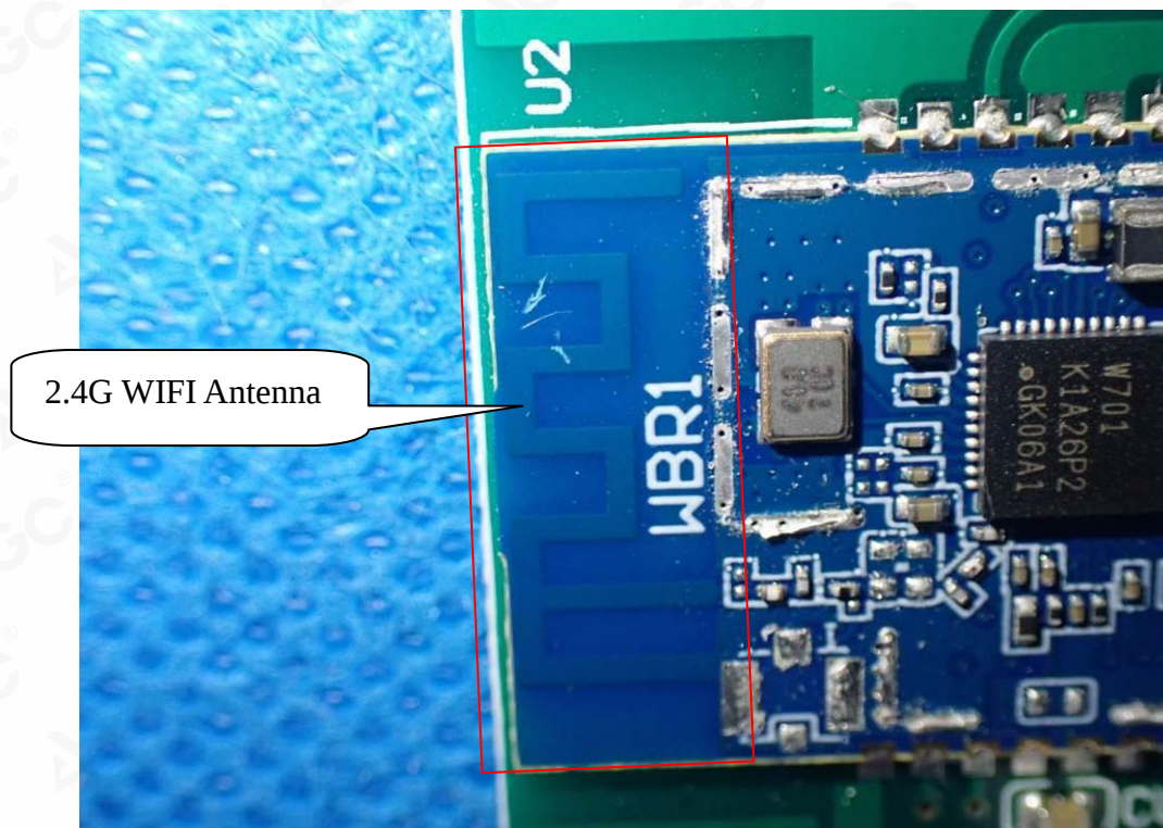
INTERNAL VIEW-19 OF EUT
