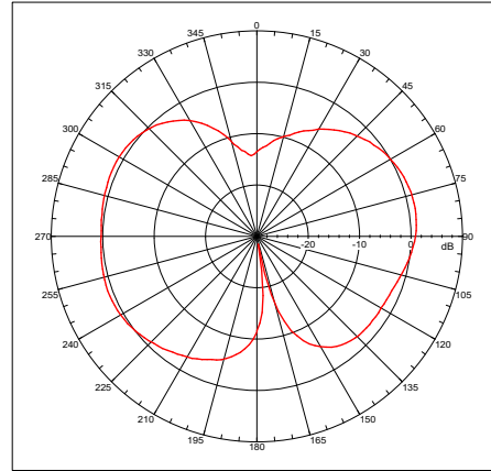
2.4GHz Gain = 1.29023 dBi Far-field amplitude of ANTENNA H.nsi
