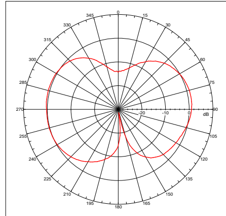
2.5GHz Gain = 1.19711 dBi
