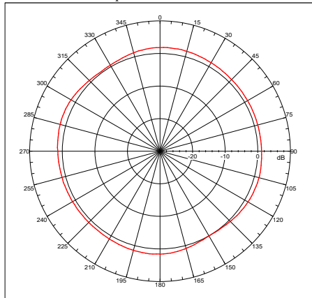
2.45GHz Gain = 1.8612 dBi Far-field amplitude of ANTENNA V.nsi
