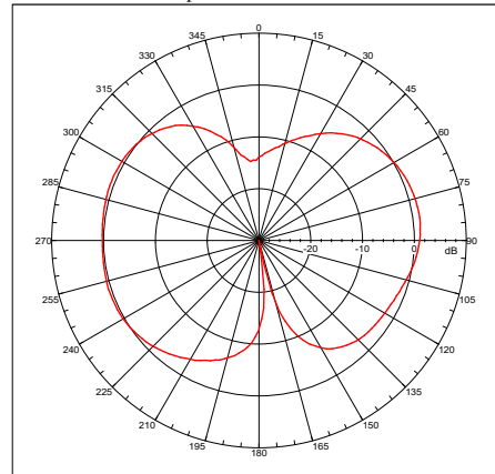
2.45GHz Gain = 1.3372 dBi Far-field amplitude of ANTENNA H.nsi
