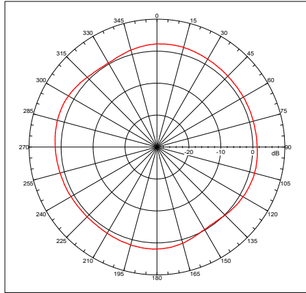
2.4GHz Gain = 2.31578 dBi Far-field amplitude of ANTENNA V.nsi
