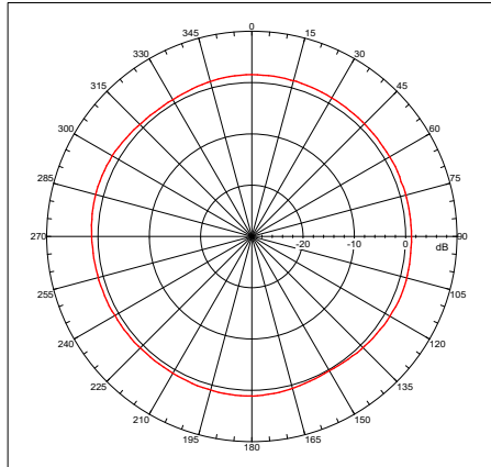
2.5GHz Gain = 1.54579 dBi
