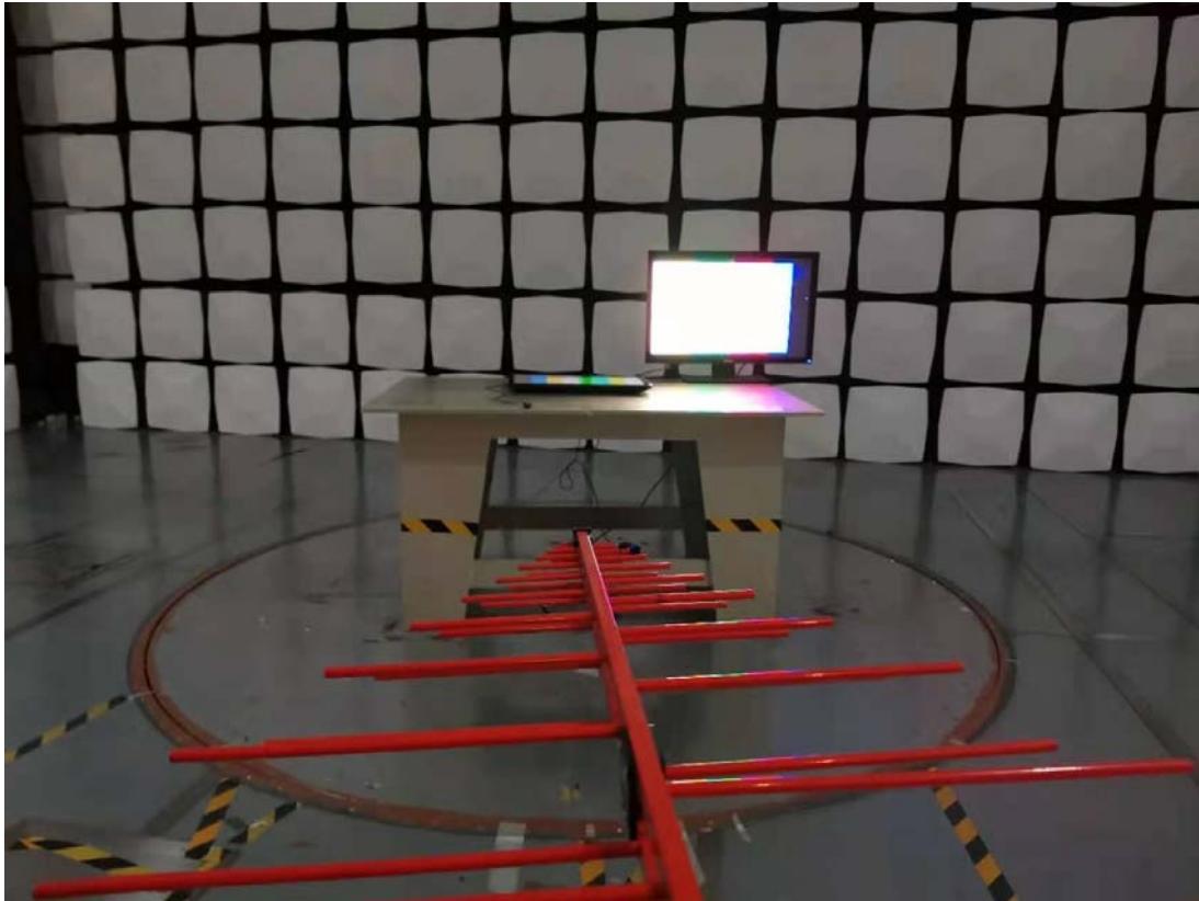
Radiated Emission Below 1GHz View MGYR10
