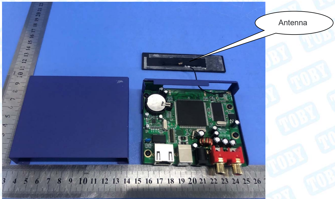
Photo 8 Internal of PCB
