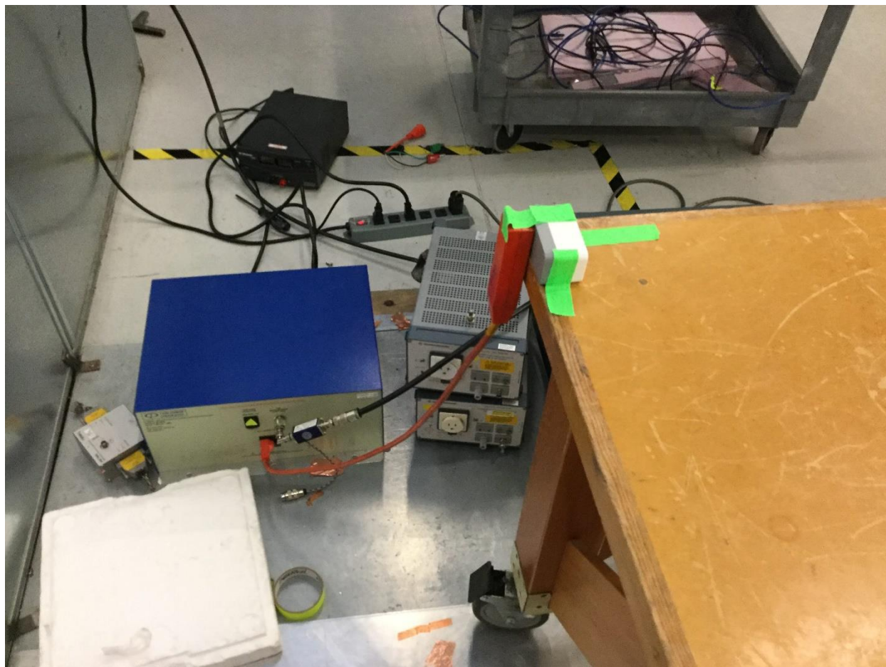
Conducted Emissions
