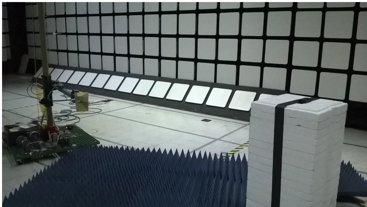
Figure 1 - Radiated Emissions Test Setup, 1 - 25 GHz, (EUT not shown)
