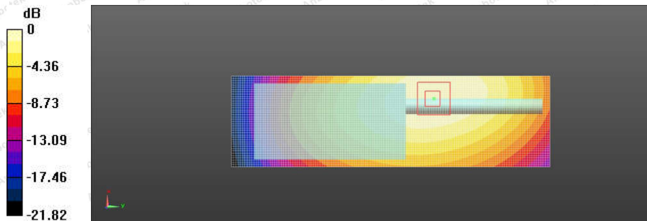
Figure 34: PMR_FM12.5KHz_Body Worn_0mm
