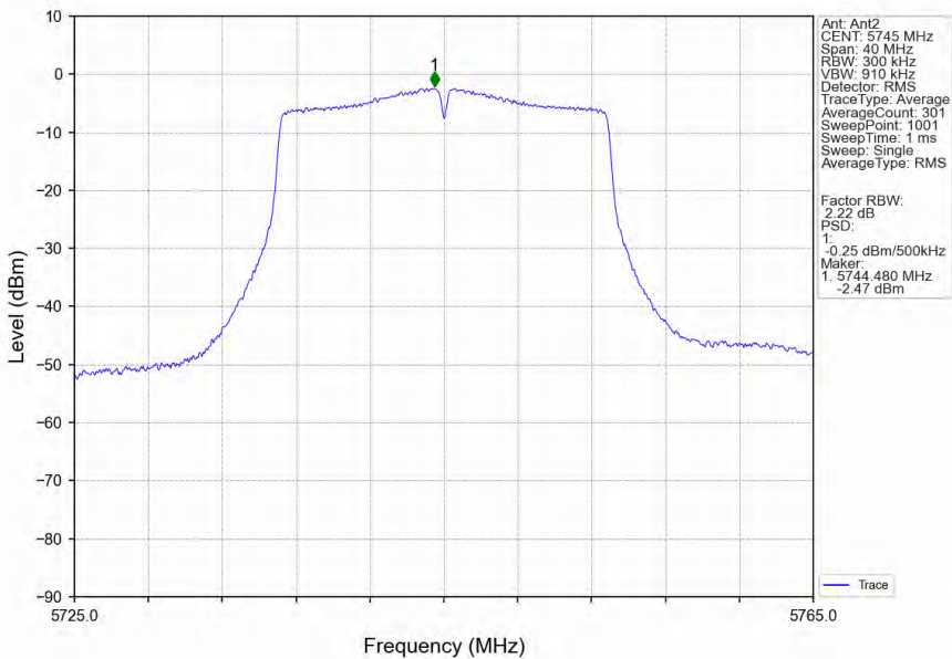
802.11n(HT20)_LCH_5745MHz_Ant2_NTNV
