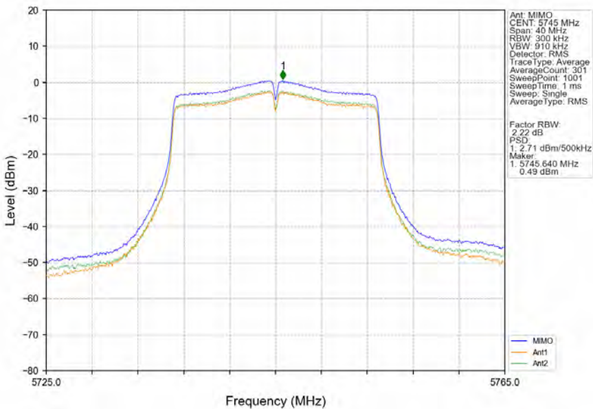
802.11n(HT20)_LCH_5745MHz_MIMO_NTNV
