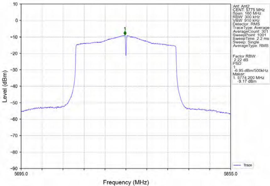
802.11ac(VHT80)_MCH_5775MHz_Ant2_NTNV
