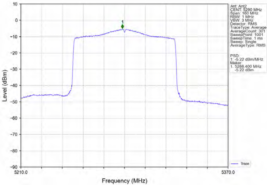
802.11ax(HEW80)_MCH_5290MHz_SU_/_Ant2_NTNV
