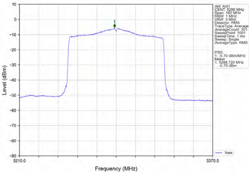
802.11ax(HEW80)_MCH_5290MHz_SU_/_Ant1_NTNV
