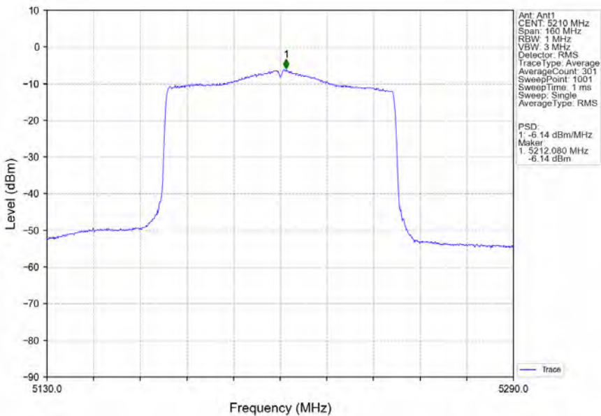
802.11ax(HEW80)_MCH_5210MHz_SU_/_Ant1_NTNV
