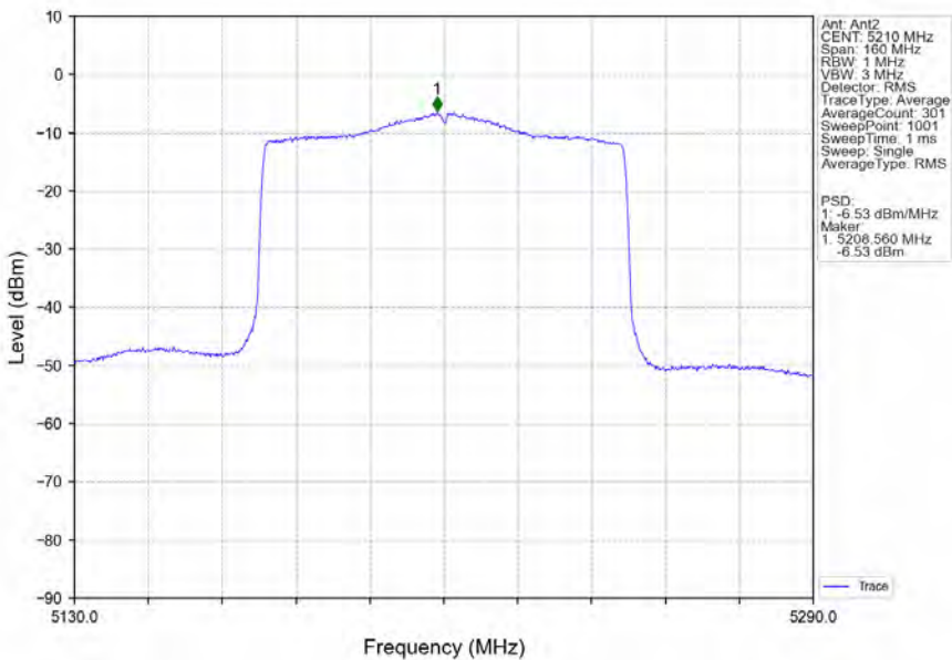
802.11ax(HEW80)_MCH_5210MHz_SU_/_Ant2_NTNV
