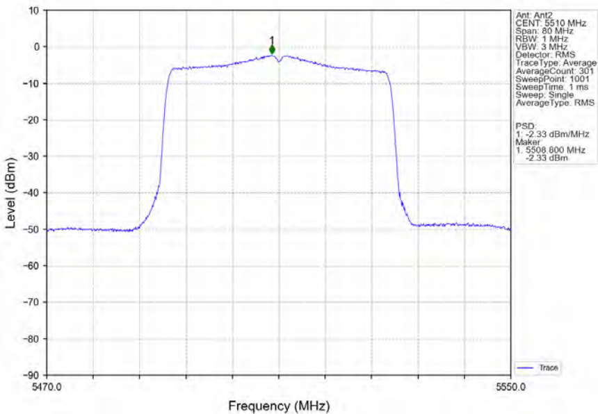
802.11ax(HEW40)_LCH_5510MHz_SU_ / _Ant2_NTNV
