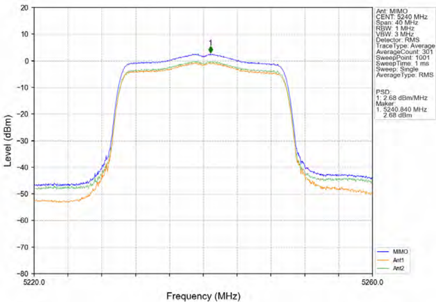
802.11ax(HEW20)_HCH_5240MHz_SU_/_MIMO_NTNV
