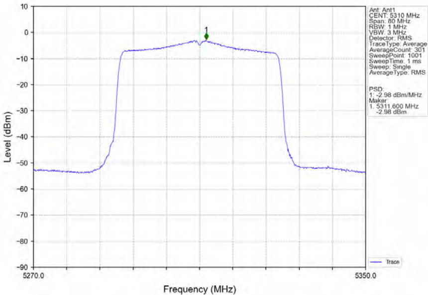
802.11ax(HEW40)_HCH_5310MHz_SU_/_Ant1_NTNV
