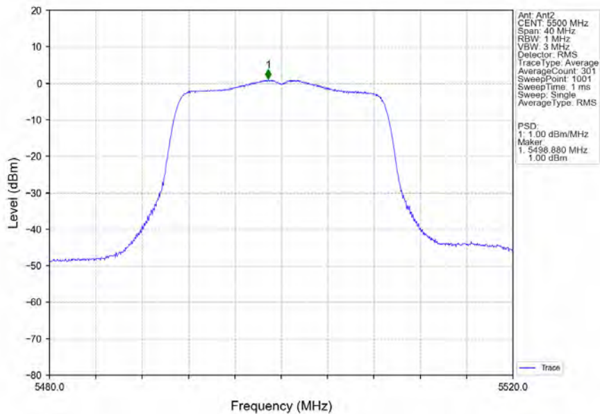
802.11ac(VHT20)_LCH_5500MHz_Ant2_NTNV
