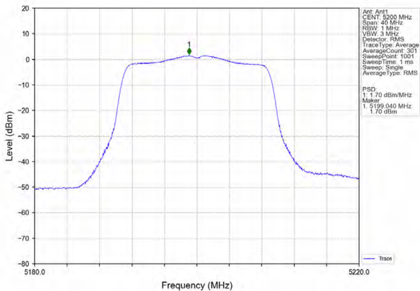
802.11n(HT20)_MCH_5200MHz_Ant1_NTNV
