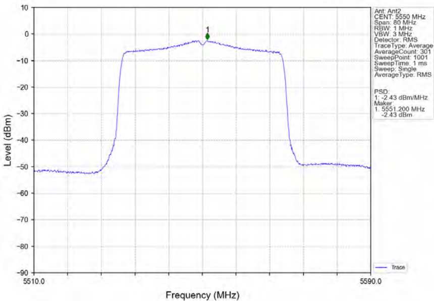
802.11ax(HEW40)_MCH_5550MHz_SU_/_Ant2_NTNV
