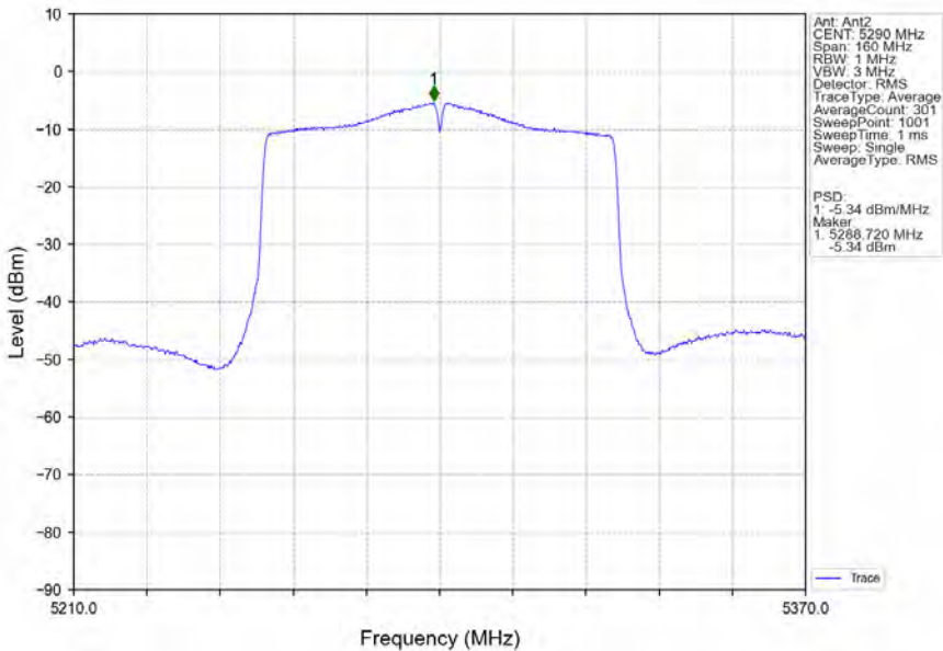
802.11ac(VHT80)_MCH_5290MHz_Ant2_NTNV
