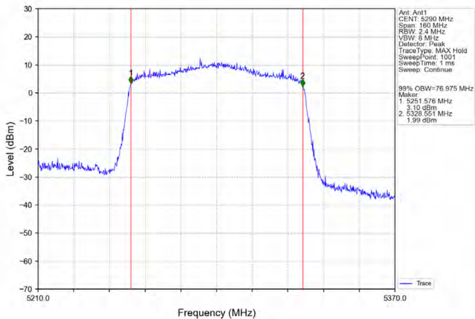
802.11ax(HEW80)_MCH_5290MHz_SU_/_Ant1_NTNV
