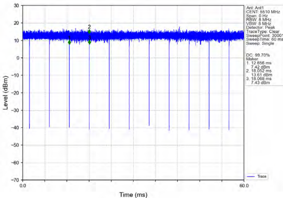
802.11ac(VHT40)_LCH_5510MHz_Ant1_NTNV
