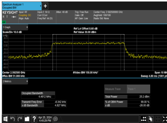
N38(5M)_CP-OFDM_64 QAM_Outer_Full_Mid_CH
