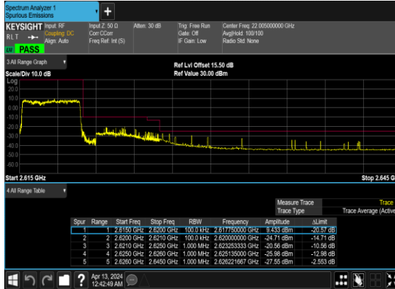
N38(5M)_DFT-s- OFDM_BPSK_Outer_Full_High_CH
