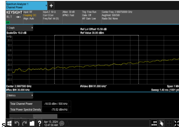
N38(25M)_DFT-s- OFDM_QPSK_Edge_1RB_Left_Low_CH_chp_pas
