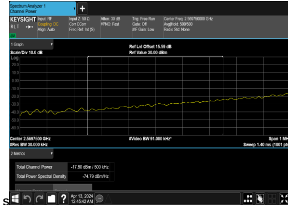
N38(25M)_DFT-s- OFDM_BPSK_Edge_1RB_Left_Low_CH_chp_pas
