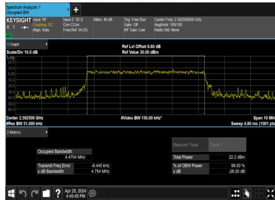
N38(5M)_CP-OFDM_256 QAM_Outer_Full_Mid_CH
