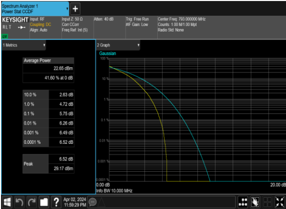
N14(10M)_DFT-s-OFDM_QPSK_Outer_Full_Mid_CH
