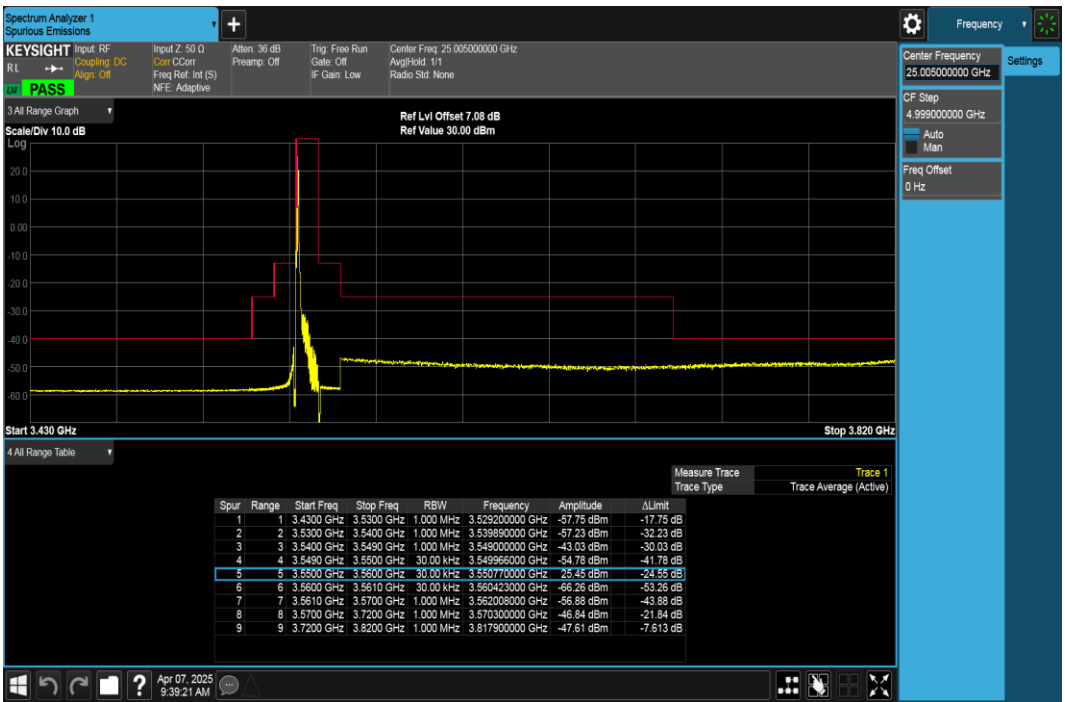
N48-10M-MASK-LCH-DFT-s-OFDM-Pi2 BPSK-1RB0
