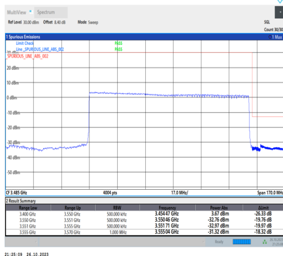
1-N78-3450-3550-PC2-30-100-H-3-DFT-PI2BPSK-Outer_Full-270@0-Ant0-1--PASS-see graph
