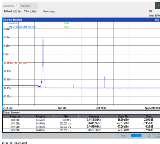
1-N78-3450-3550-PC2-30-80-L-4-CP-QPSK-Edge_1RB_Left-1@0-Ant0-1--PASS-see graph
