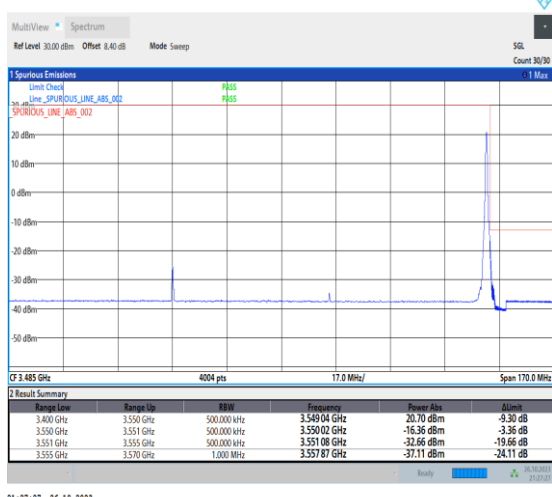
1-N78-3450-3550-PC2-30-100-H-5-CP-QPSK-Edge_1RB_Right-1@272-Ant0-1--PASS-see graph
