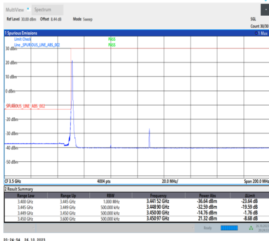
1-N78-3450-3550-PC2-30-60-L-4-CP-QPSK-Edge_1RB_Left-1@0-Ant0-1--PASS-see graph
