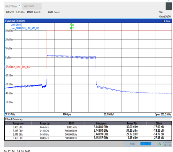
1-N78-3450-3550-PC2-30-60-L-6-CP-QPSK-Outer_Full-162@0-Ant0-1--PASS-see graph
