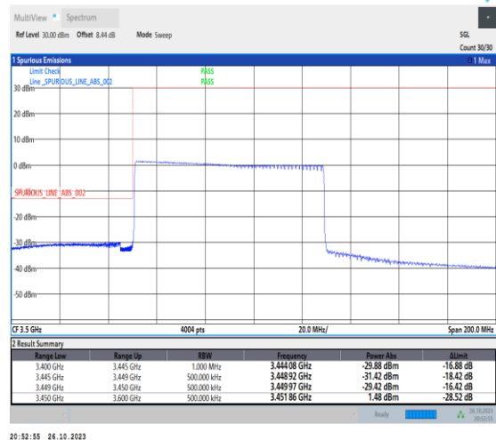
1-N78-3450-3550-PC2-30-80-L-6-CP-QPSK-Outer_Full-217@0-Ant0-1--PASS-see graph
