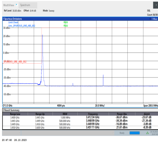
1-N78-3450-3550-PC2-30-80-L-1-DFT-PI2BPSK-Edge_1RB_Left-1@0-Ant0-1--PASS-see graph
