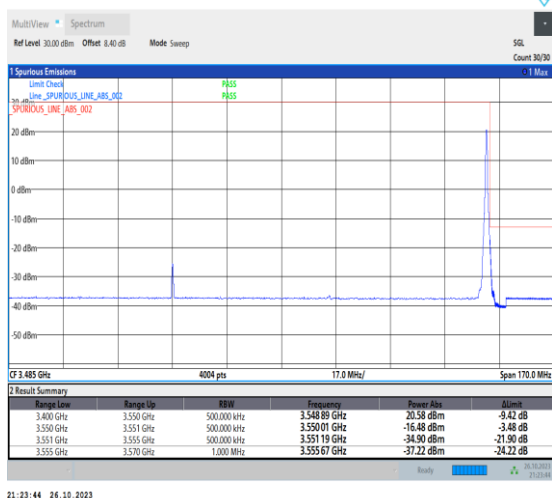
1-N78-3450-3550-PC2-30-100-H-2-DFT-PI2BPSK-Edge_1RB_Right-1@272-Ant0-1--PASS-see graph
