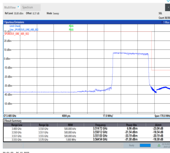
1-N78-3450-3550-PC2-30-40-H-3-DFT-PI2BPSK-Outer_Full-100@0-Ant0-1--PASS-see graph
