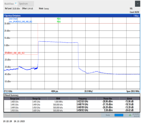
1-N78-3450-3550-PC2-30-60-L-3-DFT-PI2BPSK-Outer_Full-162@0-Ant0-1--PASS-see graph
