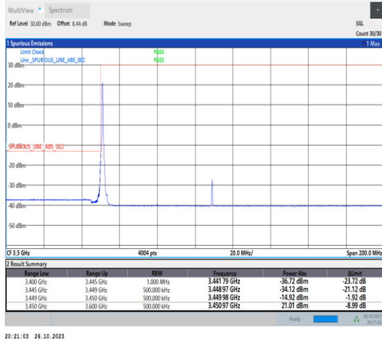
1-N78-3450-3550-PC2-30-60-L-1-DFT-PI2BPSK-Edge_1RB_Left-1@0-Ant0-1--PASS-see graph
