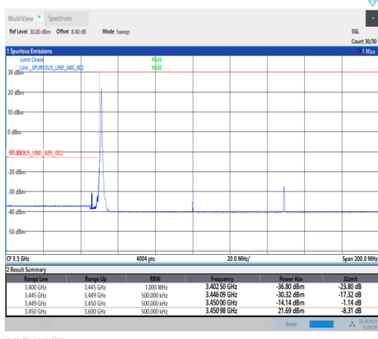
1-N78-3450-3550-PC2-30-100-L-4-CP-QPSK-Edge_1RB_Left-1@0-Ant0-1--PASS-see graph
