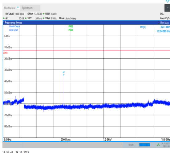
1-N78-3450-3550-PC2-30-100-M-1-DFT-PI2BPSK-I nner_1RB_Left-1@1-6000-18000-Ant0-10354.08--3 5.51--13-PASS
