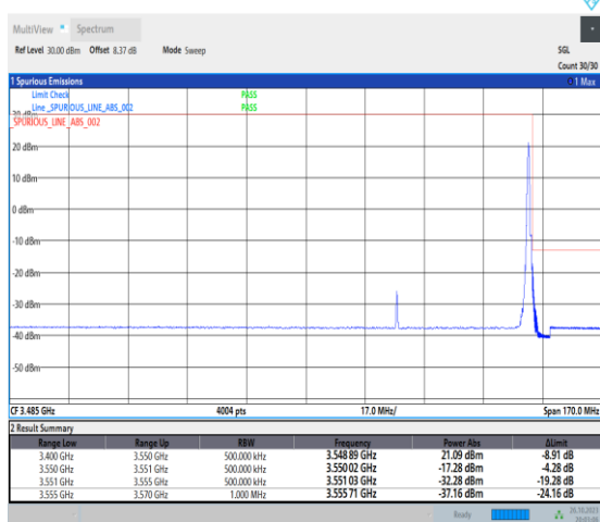
1-N78-3450-3550-PC2-30-40-H-5-CP-QPSK-Edge_1RB_Right-1@105-Ant0-1--PASS-see graph
