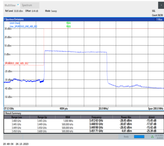
1-N78-3450-3550-PC2-30-80-L-3-DFT-PI2BPSK-Outer_Full-216@0-Ant0-1--PASS-see graph
