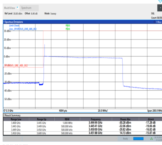
1-N78-3450-3550-PC2-30-100-L-6-CP-QPSK-Outer_Full-273@0-Ant0-1--PASS-see graph
