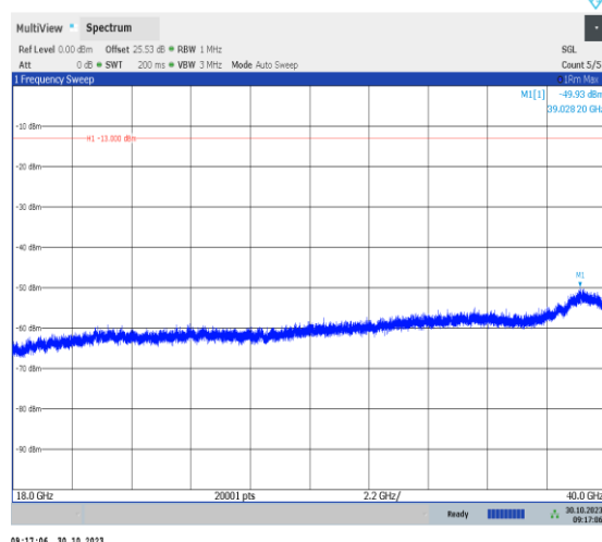
1-N78-3450-3550-PC2-30-100-M-1-DFT-PI2BPSK-In ner_1RB_Left-1@1-18000-40000-Ant0-18000.00--58 .05--13-PASS
