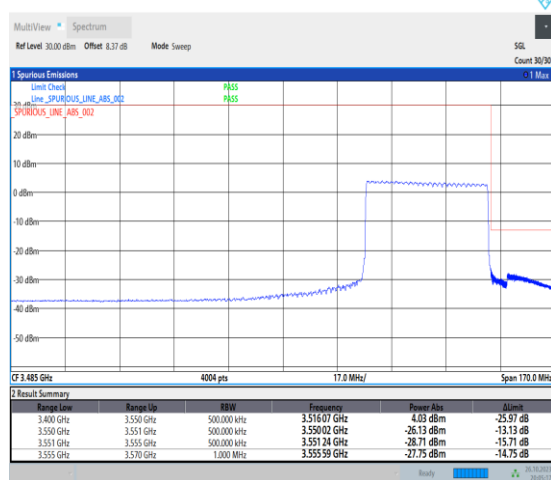
1-N78-3450-3550-PC2-30-40-H-6-CP-QPSK-Outer_Full-106@0-Ant0-1--PASS-see graph
