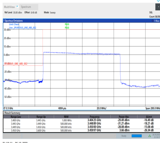
1-N78-3450-3550-PC2-30-100-L-3-DFT-PI2BPSK-Outer_Full-270@0-Ant0-1--PASS-see graph
