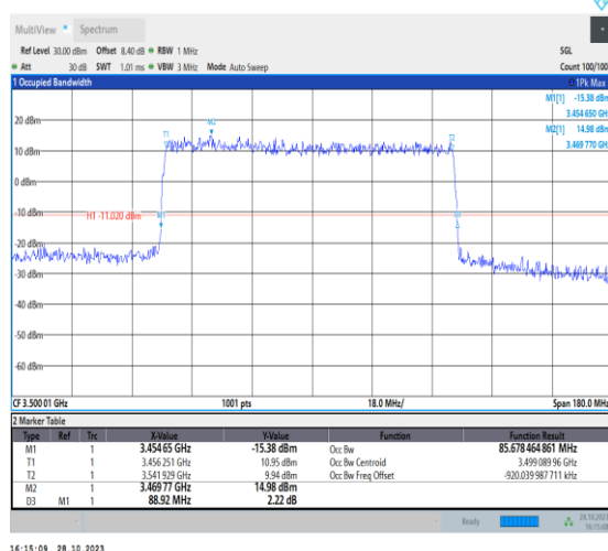
1-N78-3450-3550-PC2-30-90-M-3-DFT-16QAM-Outer _Full-240@0-Ant0-85.678-88.920-≤90-PASS
