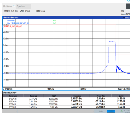
1-N78-3450-3550-PC2-30-10-H-6-CP-QPSK-Outer_Full-24@0-Ant1-1--PASS-see graph
