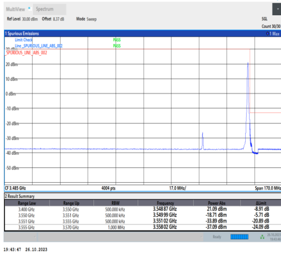
1-N78-3450-3550-PC2-30-30-H-2-DFT-PI2BPSK-Edge_1RB_Right-1@77-Ant0-1--PASS-see graph
