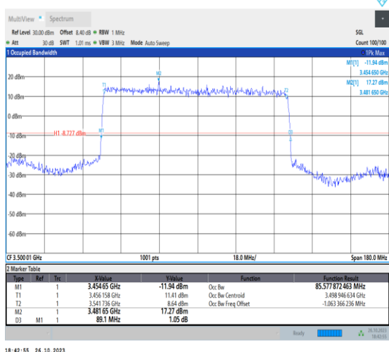
1-N78-3450-3550-PC2-30-90-M-2-DFT-PI2BPSK-Outer _Full-240@0-Ant0-85.578-89.100-≤90-PASS
