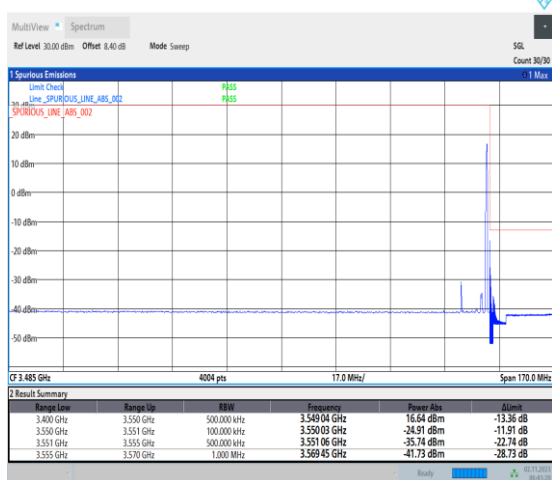
1-N78-3450-3550-PC2-30-10-H-5-CP-QPSK-Edge_1RB_Right-1@23-Ant1-1--PASS-see graph
