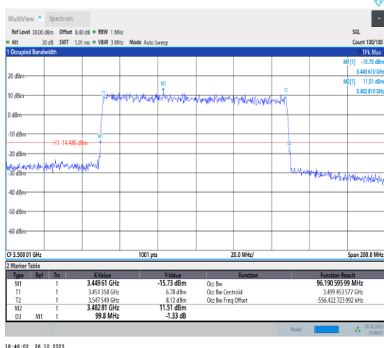
1-N78-3450-3550-PC2-30-100-M-5-DFT-256QAM-Out er_Full-270@0-Ant0-96.191-99.800-≤100-PASS
