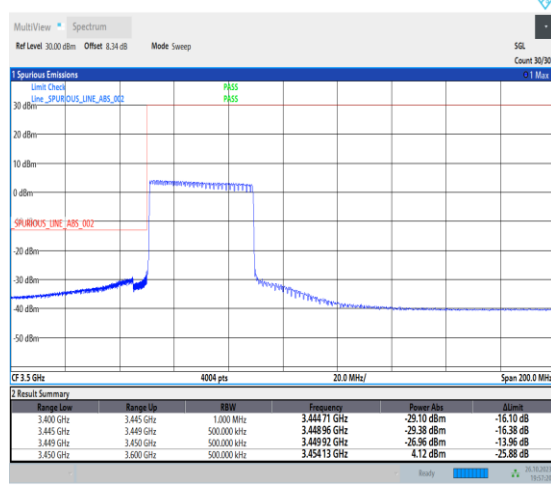
1-N78-3450-3550-PC2-30-40-L-6-CP-QPSK-Outer_Full-106@0-Ant0-1--PASS-see graph
