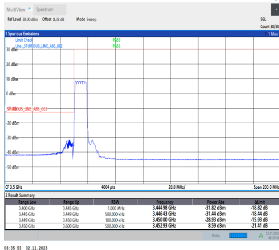
1-N78-3450-3550-PC2-30-10-L-3-DFT-PI2BPSK-Outer_Full-24@0-Ant1-1--PASS-see graph
