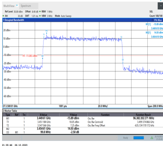
1-N78-3450-3550-PC2-30-100-M-3-DFT-16QAM-Out er_Full-270@0-Ant0-96.382-99.800-≤100-PASS
