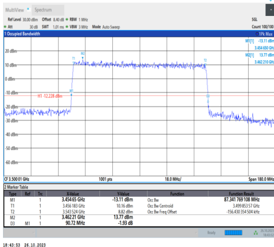
1-N78-3450-3550-PC2-30-90-M-6-CP-QPSK-Outer_Full-245@0-Ant0-87.342-90.720-≤90-PASS
