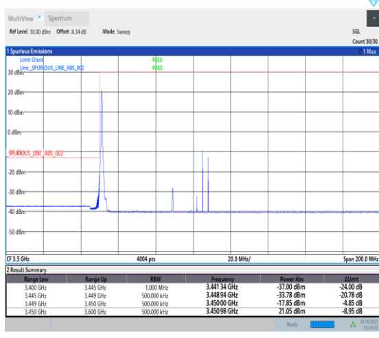
1-N78-3450-3550-PC2-30-40-L-4-CP-QPSK-Edge_1RB_Left-1@0-Ant0-1--PASS-see graph
