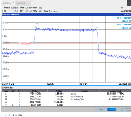
1-N78-3450-3550-PC2-30-90-M-4-DFT-64QAM-Outer_Full-240@0-Ant0-85.612-88.740-≤90-PASS
