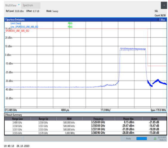
1-N78-3450-3550-PC2-30-30-H-3-DFT-PI2BPSK-Outer_Full-75@0-Ant0-1--PASS-see graph
