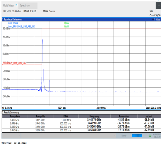
1-N78-3450-3550-PC2-30-10-L-4-CP-QPSK-Edge_1RB_Left-1@0-Ant1-1--PASS-see graph
