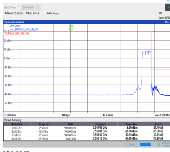
1-N78-3450-3550-PC2-30-10-H-3-DFT-PI2BPSK-Outer_Full-24@0-Ant1-1--PASS-see graph
