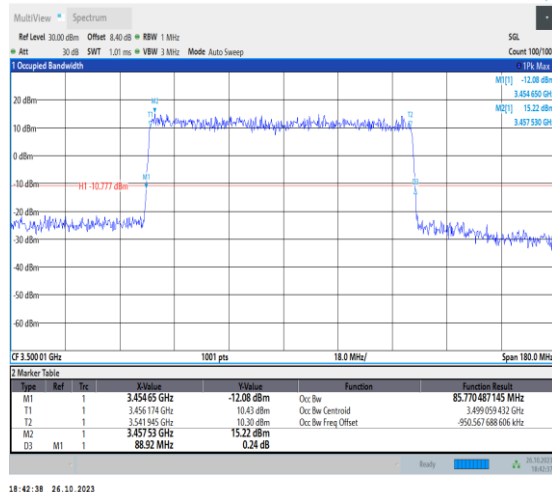
1-N78-3450-3550-PC2-30-90-M-1-DFT-QPSK-Outer _Full-240@0-Ant0-85.77-88.920-≤90-PASS
