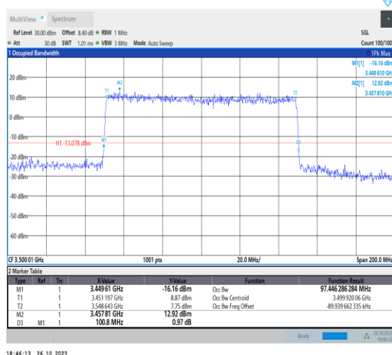
1-N78-3450-3550-PC2-30-100-M-6-CP-QPSK-Outer _Full-273@0-Ant0-97.446-100.800-≤100-PASS
