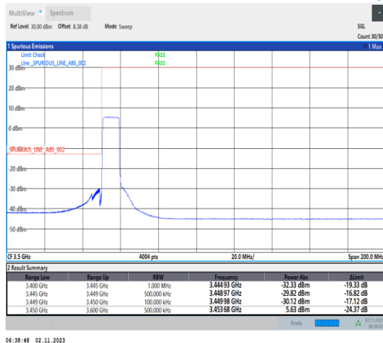
1-N78-3450-3550-PC2-30-10-L-6-CP-QPSK-Outer_Full-24@0-Ant1-1--PASS-see graph
