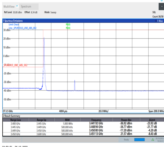
1-N78-3450-3550-PC2-30-40-L-1-DFT-PI2BPSK-Edge_1RB_Left-1@0-Ant0-1--PASS-see graph
