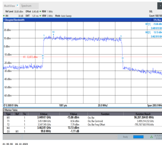
1-N78-3450-3550-PC2-30-100-M-4-DFT-64QAM-Out er_Full-270@0-Ant0-96.261-99.800-≤100-PASS
