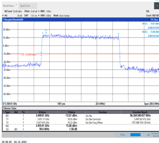
1-N78-3450-3550-PC2-30-100-M-1-DFT-QPSK-Outer_Full-270@0-Ant0-96.264-99.600-≤100-PASS
