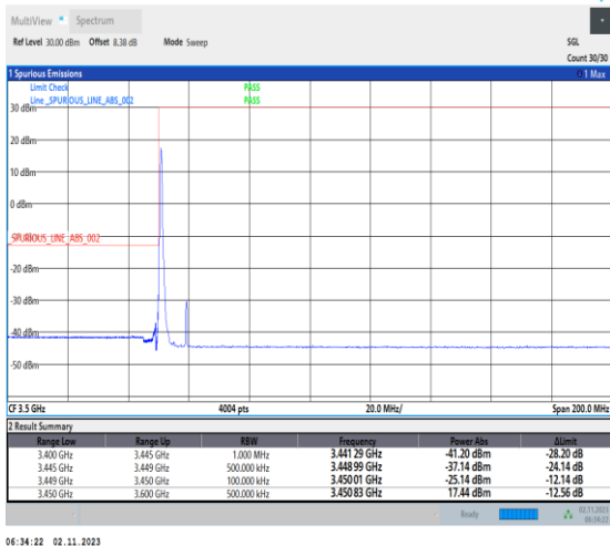
1-N78-3450-3550-PC2-30-10-L-1-DFT-PI2BPSK-Edge_1RB_Left-1@0-Ant1-1--PASS-see graph
