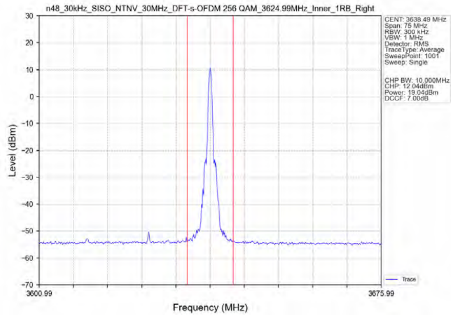
n48_30kHz_SISO_NTNV_30MHz_DFT-s-OFDM_256_QAM_3624.99MHz_Inner_1RB_Right_Ant1
