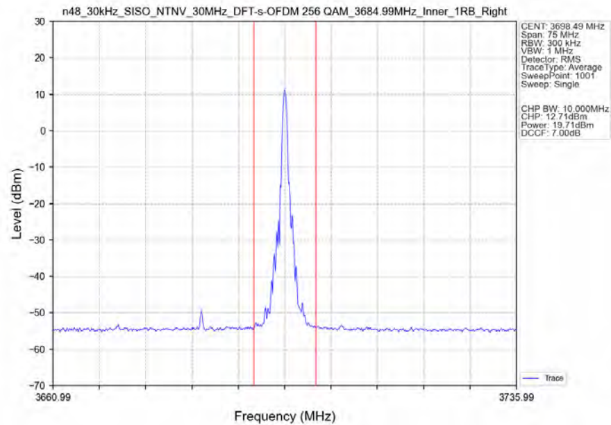
n48_30kHz_SISO_NTNV_30MHz_DFT-s-OFDM_256_QAM_3684.99MHz_Inner_1RB_Right_Ant1
