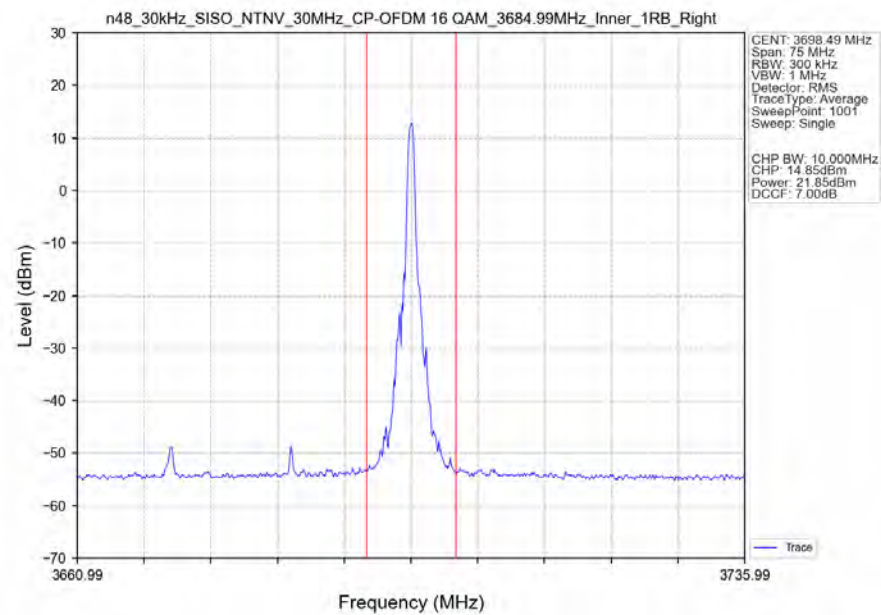
n48_30kHz_SISO_NTNV_30MHz_CP-OFDM_16_QAM_3684.99MHz_Inner_1RB_Right_Ant1
