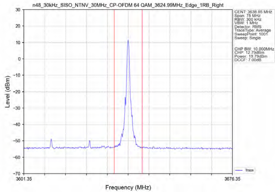
n48_30kHz_SISO_NTNV_30MHz_CP-OFDM_64_QAM_3624.99MHz_Edge_1RB_Right_Ant1
