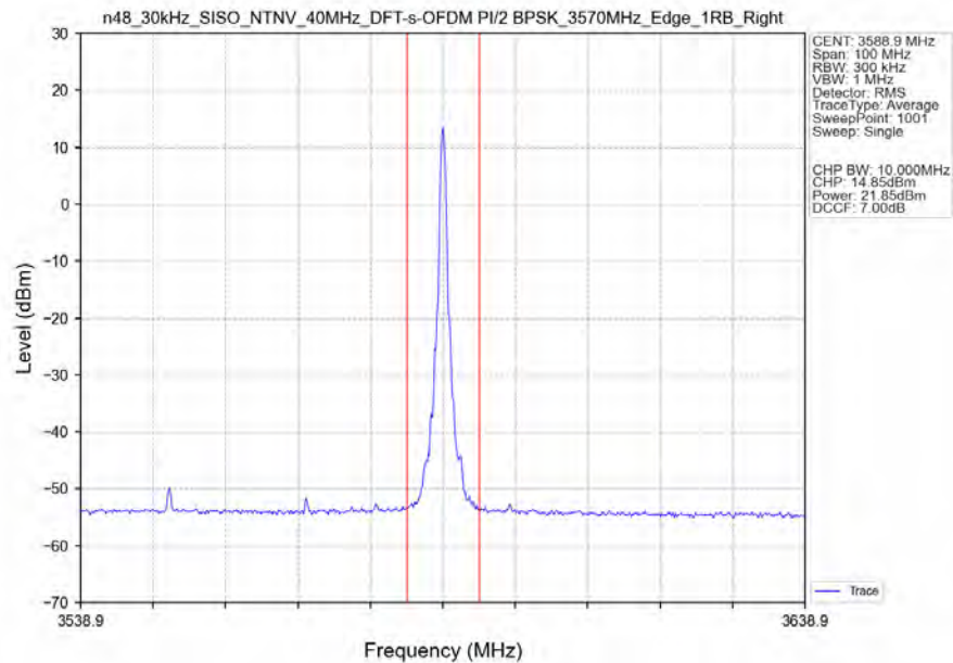
n48_30kHz_SISO_NTNV_40MHz_DFT-s-OFDM PI/2 BPSK_3570MHz_Edge_1RB_Right_Ant1
