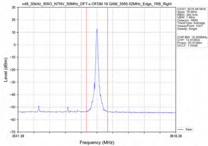
n48_30kHz_SISO_NTNV_30MHz_DFT-s-OFDM_16_QAM_3565.02MHz_Edge_1RB_Right_Ant1
