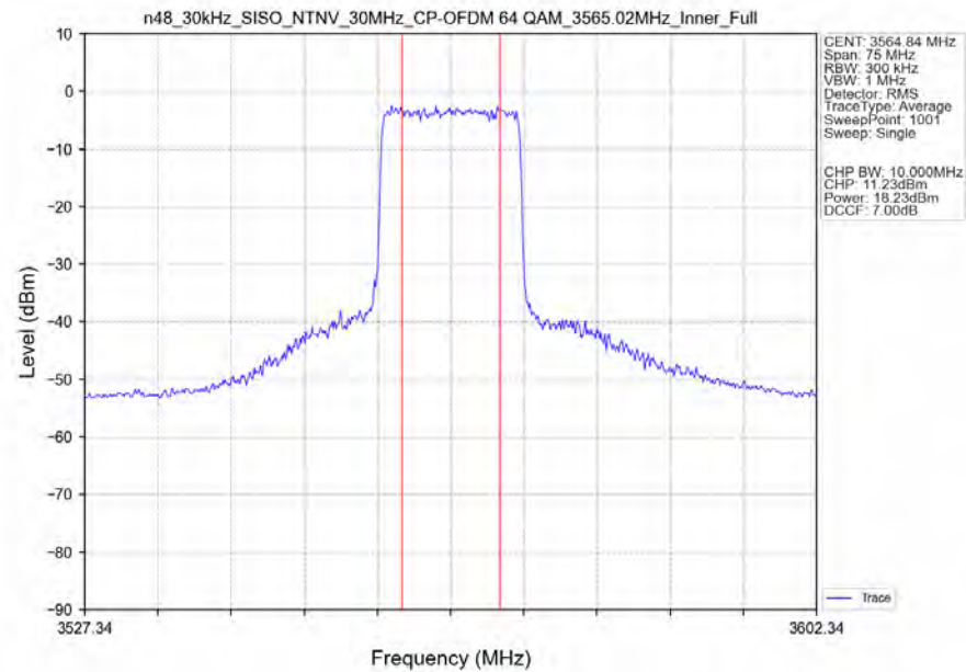
n48_30kHz_SISO_NTNV_30MHz_CP-OFDM_64_QAM_3565.02MHz_Inner_Full_Ant1
