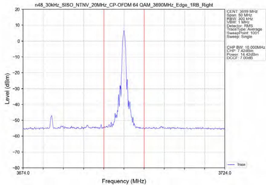
n48_30kHz_SISO_NTNV_20MHz_CP-OFDM_64_QAM_3690MHz_Edge_1RB_Right_Ant1
