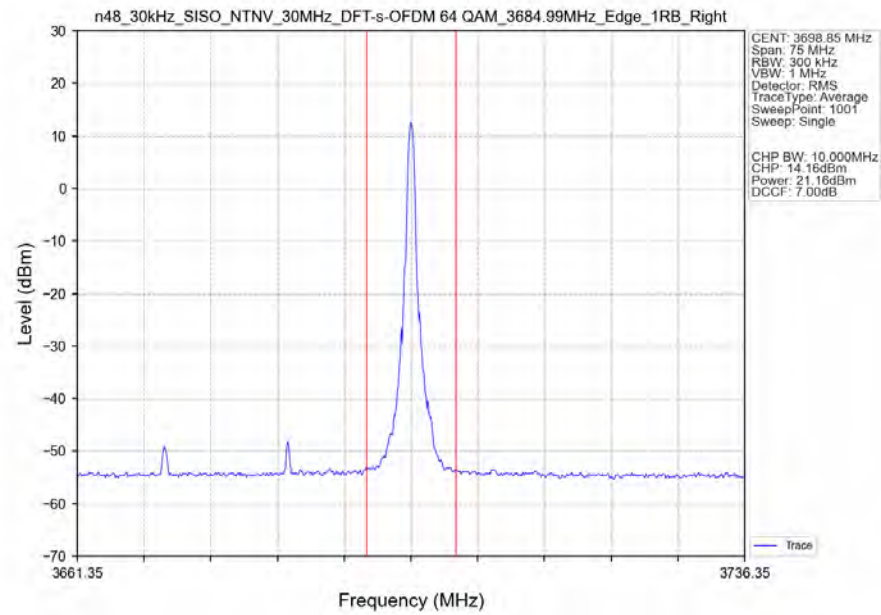
n48_30kHz_SISO_NTNV_30MHz_DFT-s-OFDM_64_QAM_3684.99MHz_Edge_1RB_Right_Ant1
