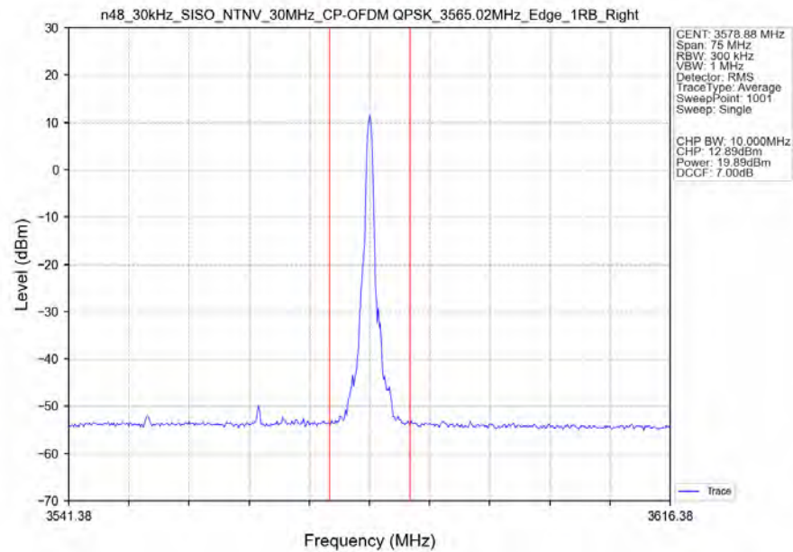
n48_30kHz_SISO_NTNV_30MHz_CP-OFDM_QPSK_3565.02MHz_Edge_1RB_Right_Ant1
