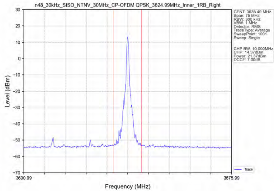
n48_30kHz_SISO_NTNV_30MHz_CP-OFDM_QPSK_3624.99MHz_Inner_1RB_Right_Ant1
