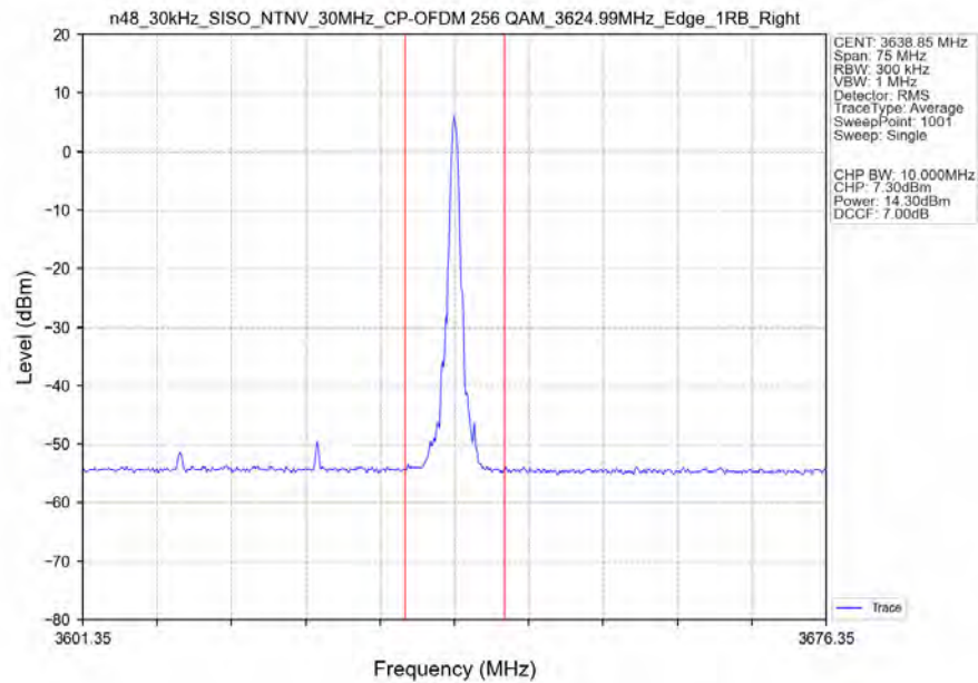
n48_30kHz_SISO_NTNV_30MHz_CP-OFDM_256_QAM_3624.99MHz_Edge_1RB_Right_Ant1
