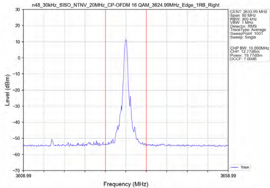
n48_30kHz_SISO_NTNV_20MHz_CP-OFDM_16_QAM_3624.99MHz_Edge_1RB_Right_Ant1
