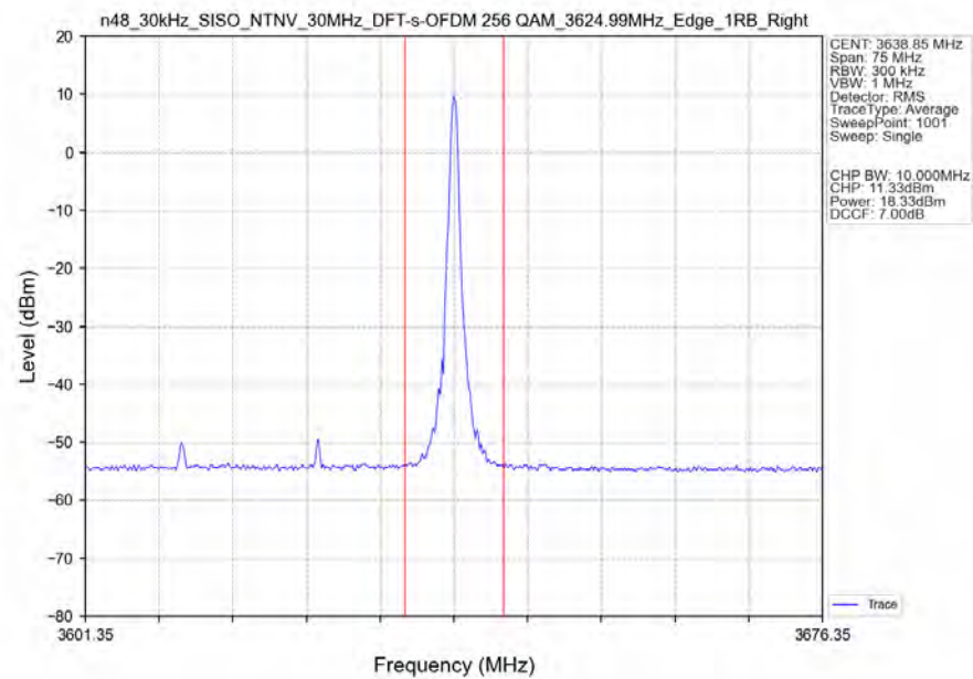
n48_30kHz_SISO_NTNV_30MHz_DFT-s-OFDM_256_QAM_3624.99MHz_Edge_1RB_Right_Ant1
