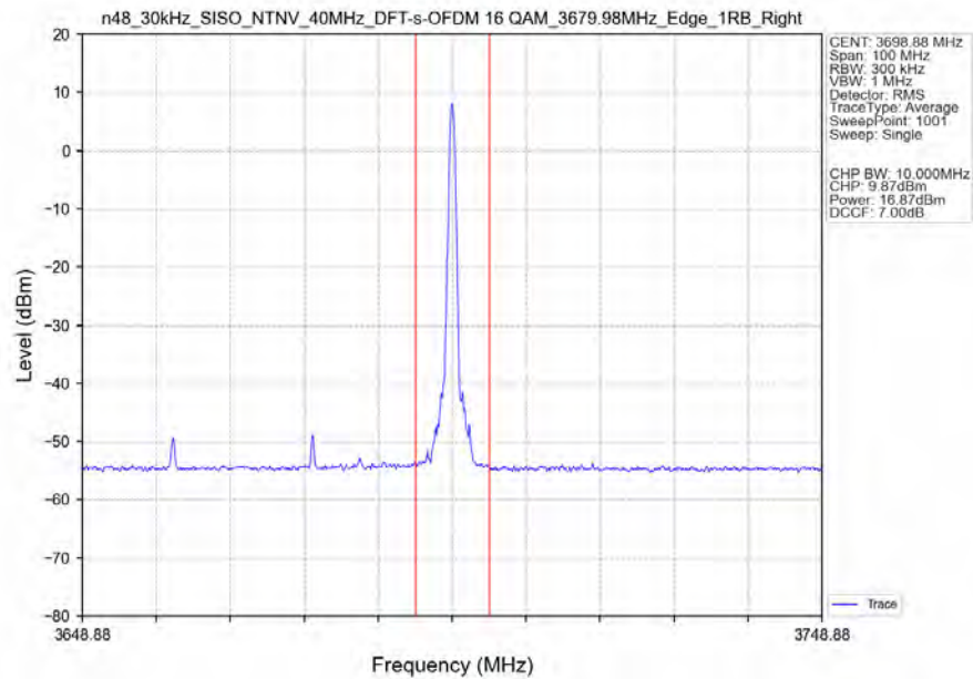
n48_30kHz_SISO_NTNV_40MHz_DFT-s-OFDM_16_QAM_3679.98MHz_Edge_1RB_Right_Ant1
