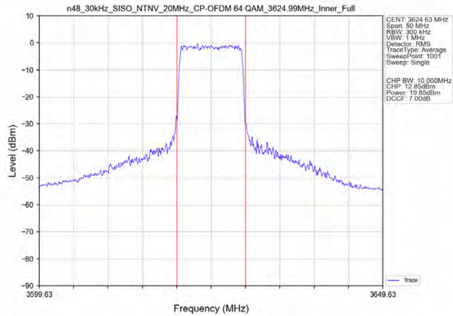
n48_30kHz_SISO_NTNV_20MHz_CP-OFDM_64_QAM_3624.99MHz_Inner_Full_Ant1
