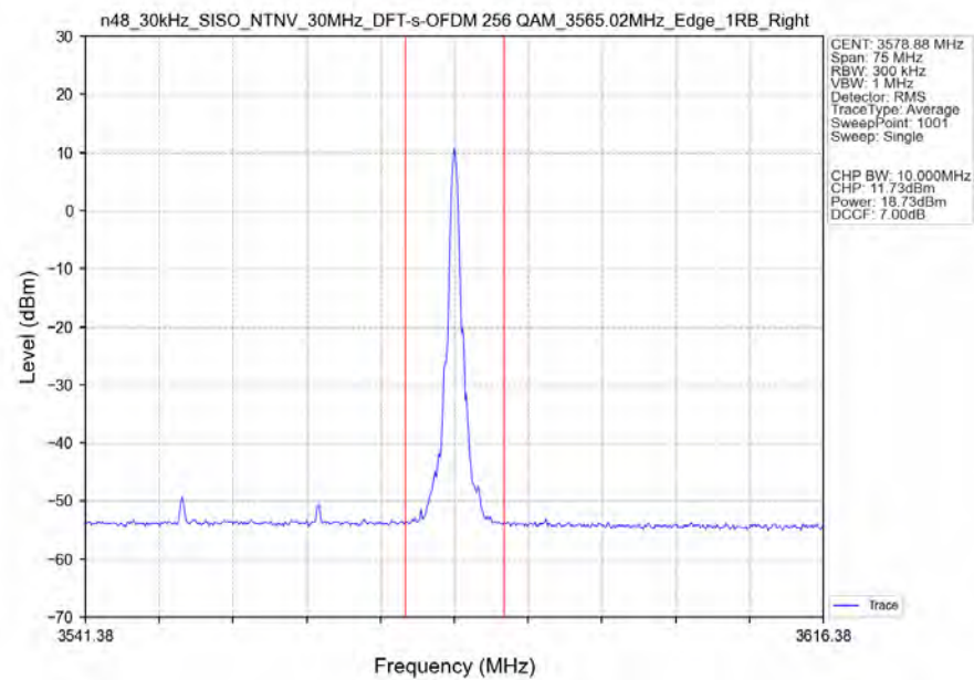
n48_30kHz_SISO_NTNV_30MHz_DFT-s-OFDM_256_QAM_3565.02MHz_Edge_1RB_Right_Ant1
