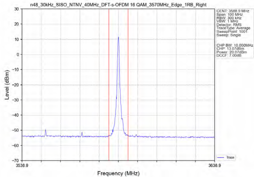
n48_30kHz_SISO_NTNV_40MHz_DFT-s-OFDM_16_QAM_3570MHz_Edge_1RB_Right_Ant1
