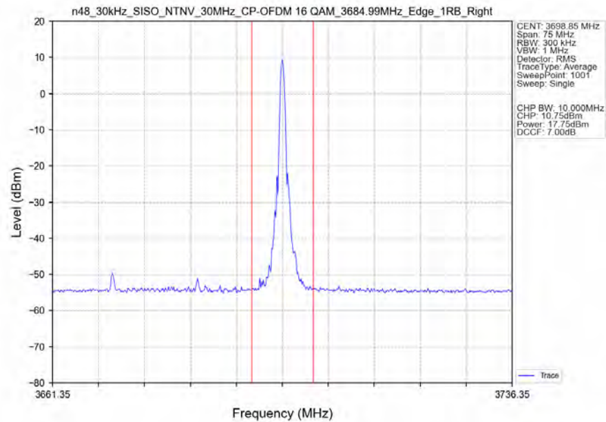
n48_30kHz_SISO_NTNV_30MHz_CP-OFDM_16_QAM_3684.99MHz_Edge_1RB_Right_Ant1
