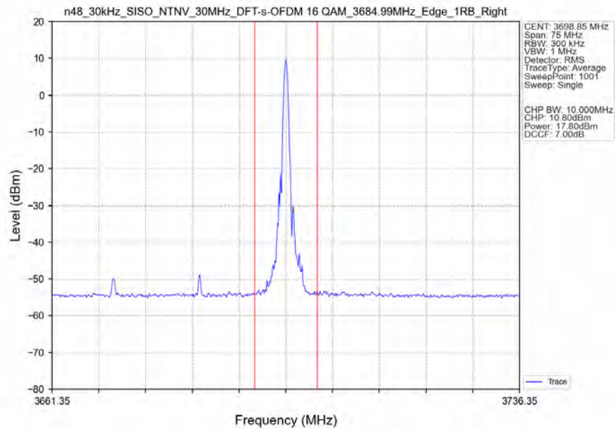
n48_30kHz_SISO_NTNV_30MHz_DFT-s-OFDM_16_QAM_3684.99MHz_Edge_1RB_Right_Ant1
