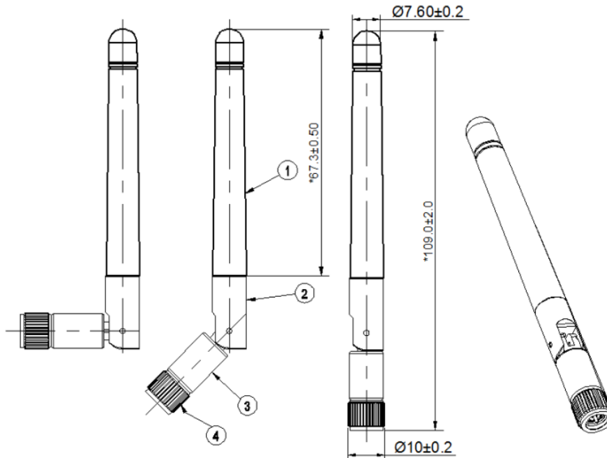
Antenna Dimensions
