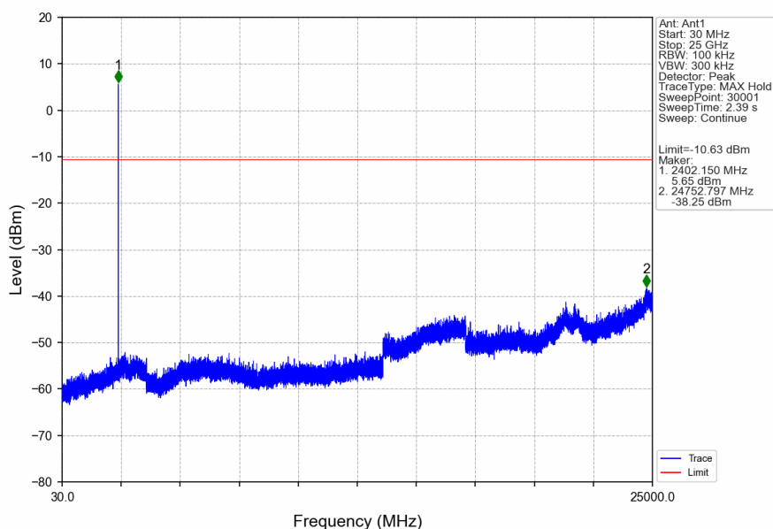
Pi/4DQPSK_2DH5_LCH_2402MHz_Ant1_NTNV
