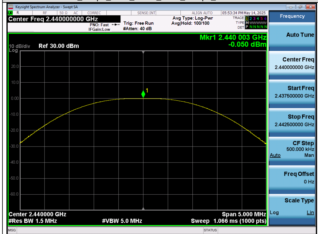
Test_Graph_2.4G_ANT1_2440_1Mbps_Peak Power
