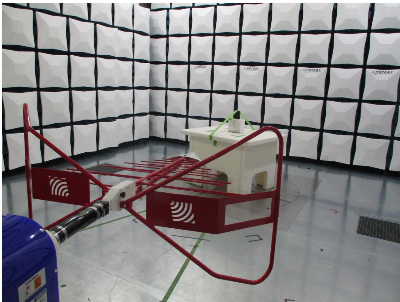
Figure 5: 30MHz-1GHz Test Setup (Front View)
