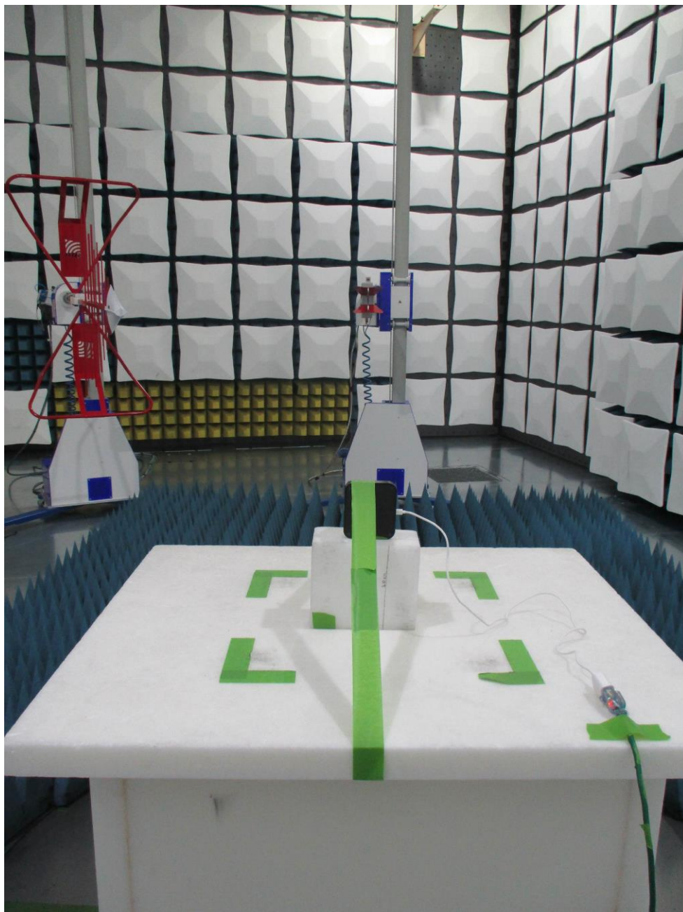
Figure 4: 1-18GHz Test Setup (Rear View)
