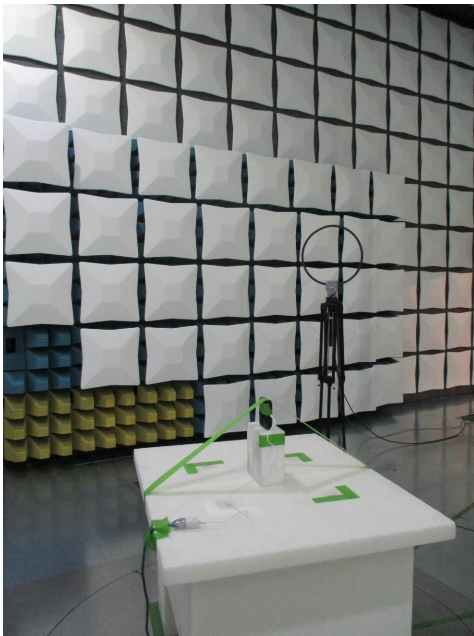
Figure 8: 9kHz-30MHz Test Setup (Rear View)
