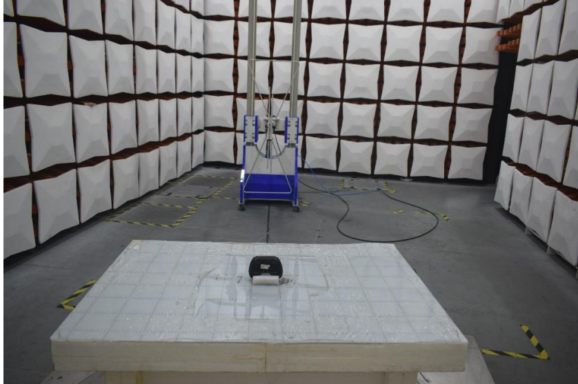
TX 30MHz~1GHz
