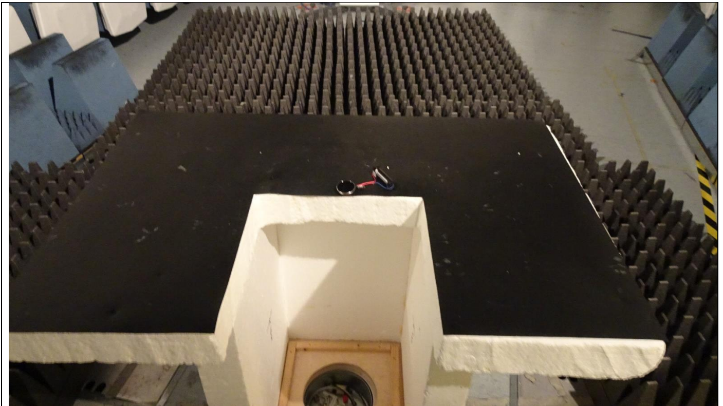
Picture 14, Radiated Spurious Emissions, EUT setup, RX 1 – 12,75 GHz
