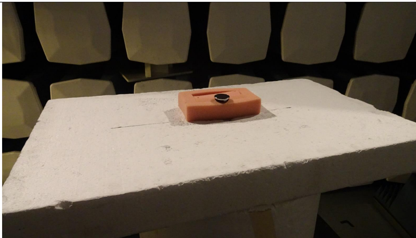
Picture 12, Radiated Spurious Emissions, EUT setup, TX 1 – 26 GHz
