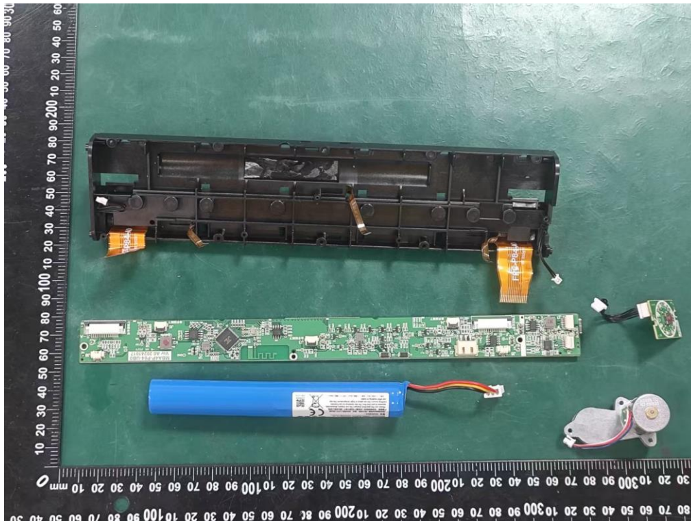
Motherboard 1
