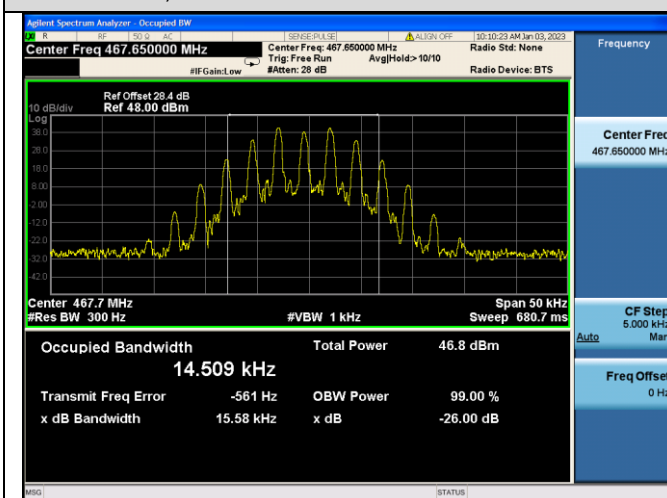
25kHz, FM Modulation:467.6500MHz-45W
