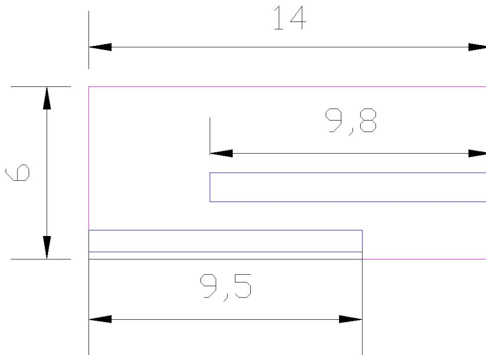
Picture of the antenna
