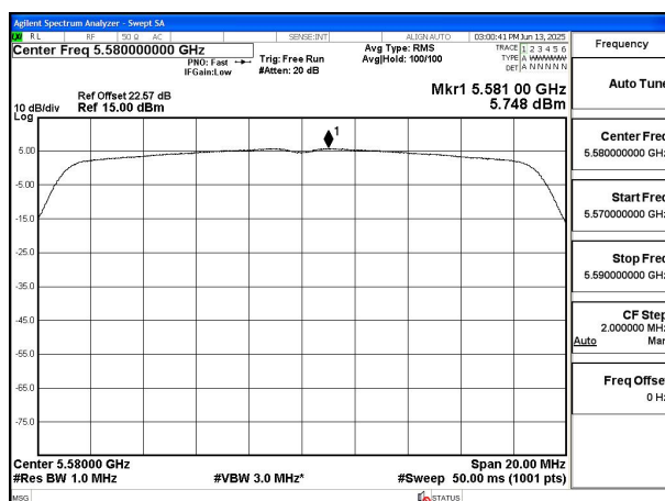
Mode:802.11ac VHT20 Frequency:5580MHz Ant:Chain1
