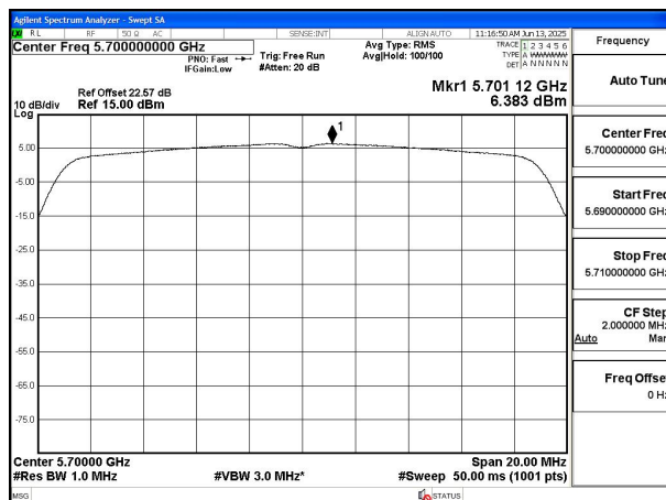
Mode:802.11ac VHT20 Frequency:5700MHz Ant:Chain0
