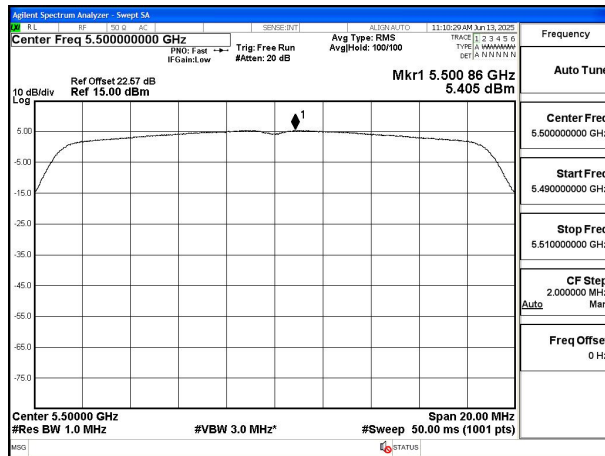
Mode:802.11ac VHT20 Frequency:5500MHz Ant:Chain0
