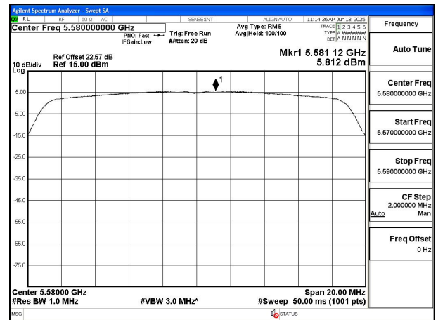
Mode:802.11ac VHT20 Frequency:5580MHz Ant:Chain0
