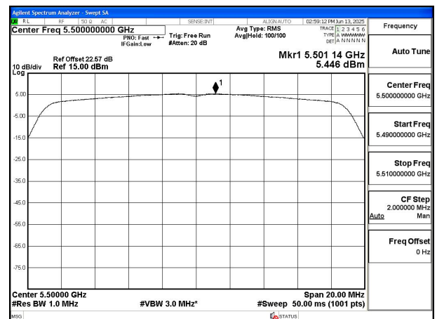
Mode:802.11ac VHT20 Frequency:5500MHz Ant:Chain1
