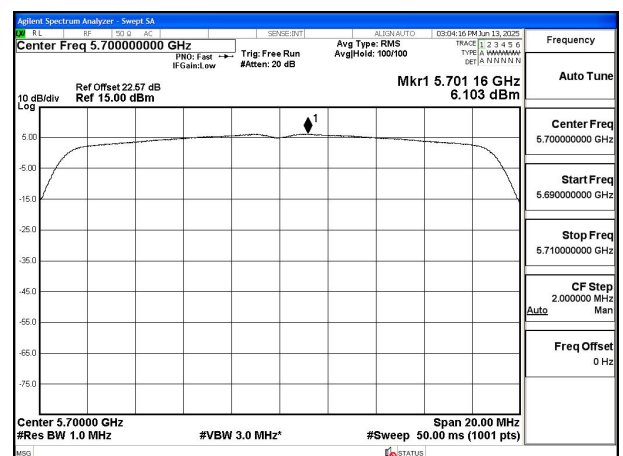
Mode:802.11ac VHT20 Frequency:5700MHz Ant:Chain1
