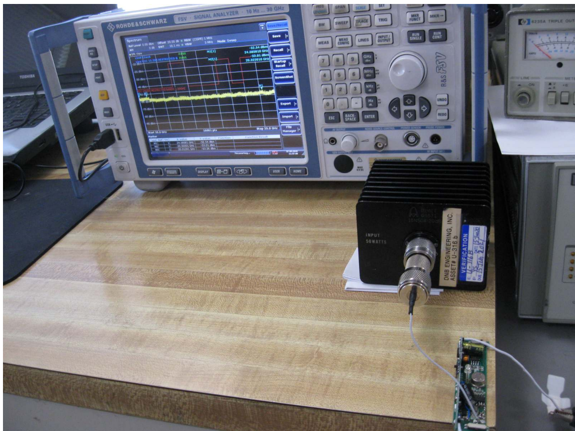
Test Set Up - Antenna Conducted Measurements
