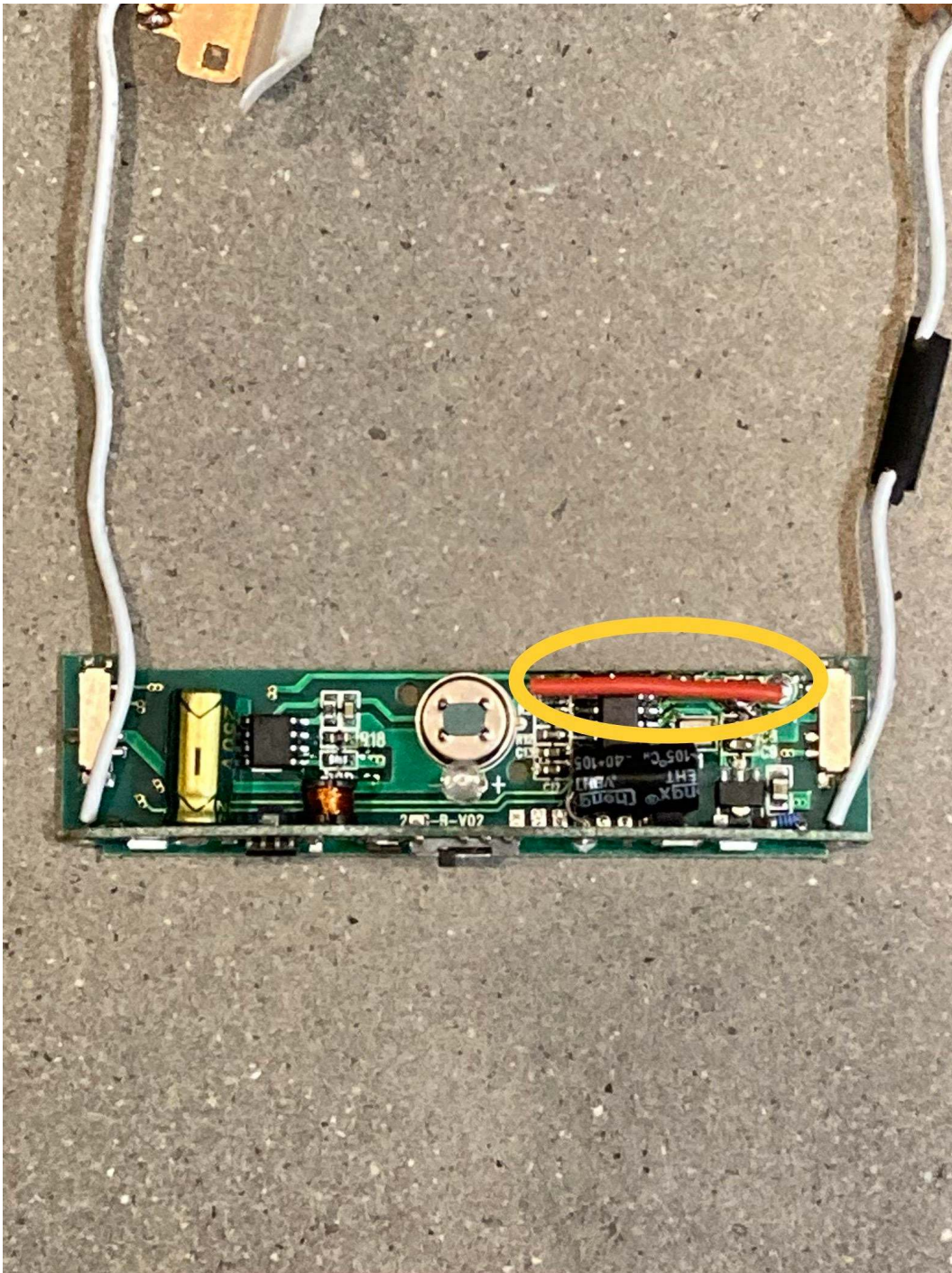
Internal Photo - unenclosed assembly with antenna and transmitter circled
