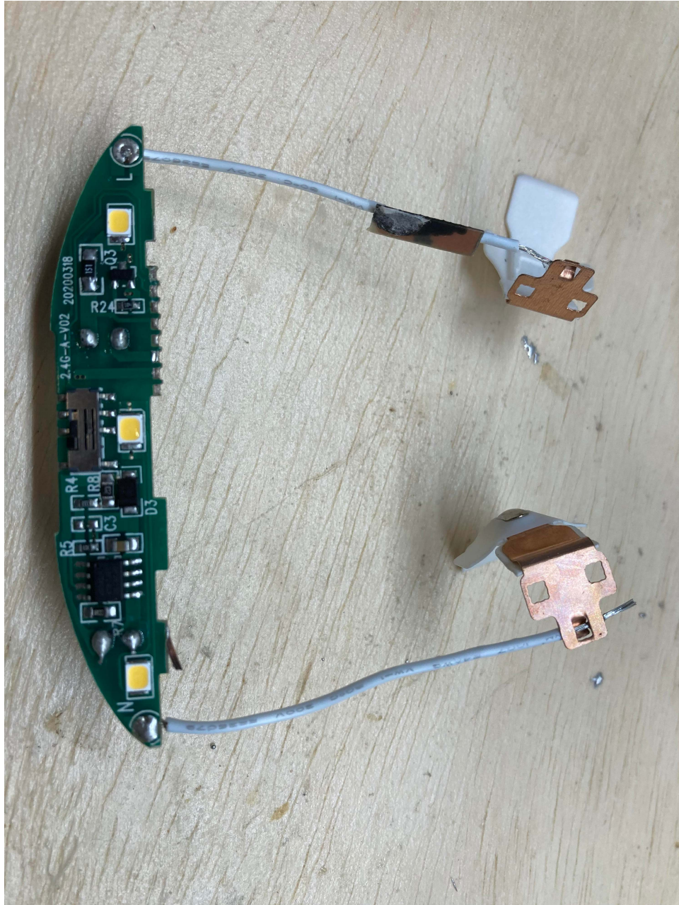
Internal photos - bare board bottom front
