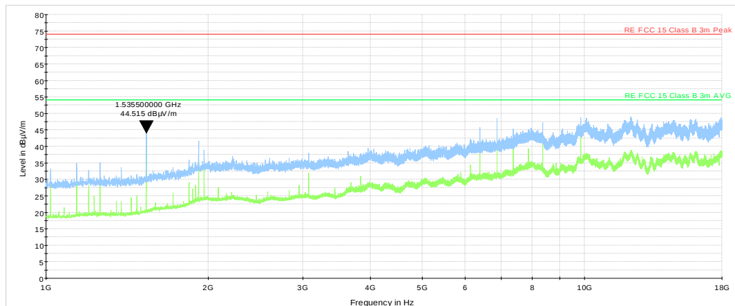
Plot 7.3.8 Radiated emission measurements from 1GHz to 18GHz at the mid carrier frequency
