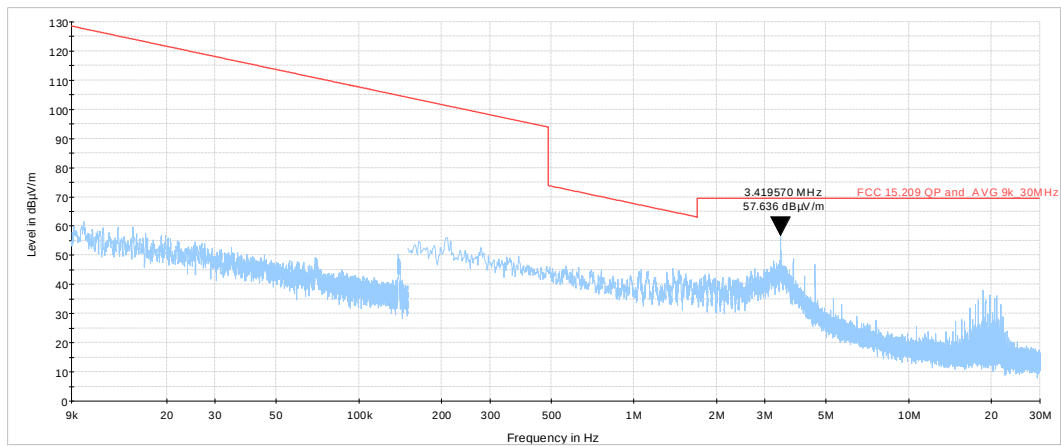
Plot 7.3.2 Radiated emission measurements from 9 KHz to 30MHz at mid carrier frequency
