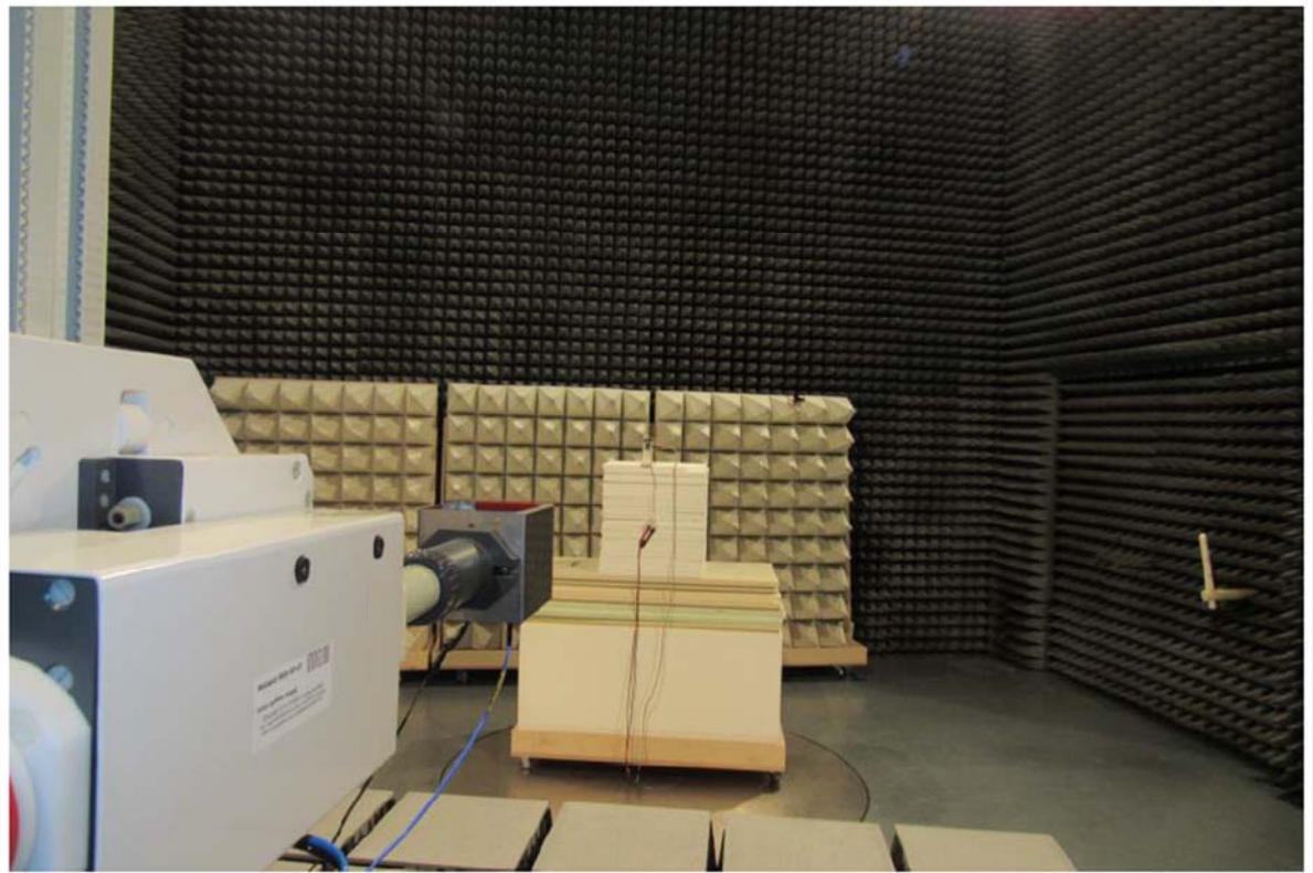
Test setup above 17 GHz
