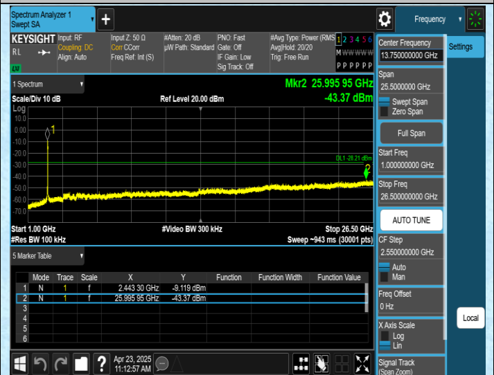
11AX40SISO-Ant1-2452-1000~26500-PASS
