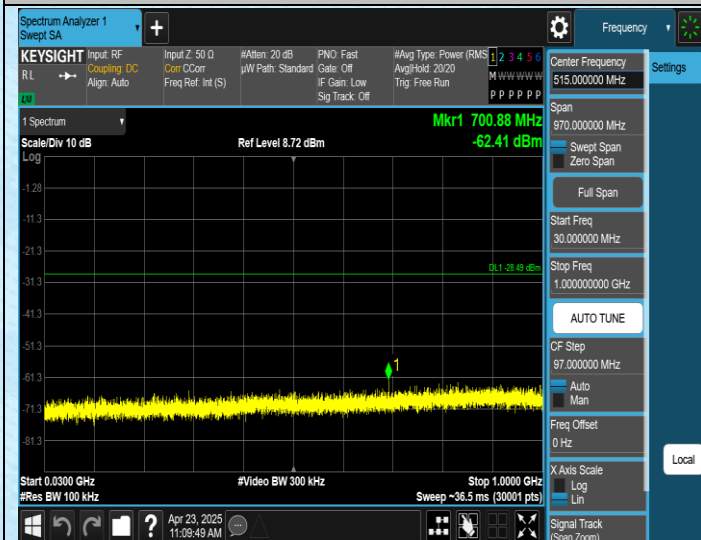
11AX40SISO-Ant1-2422-30~1000-PASS
