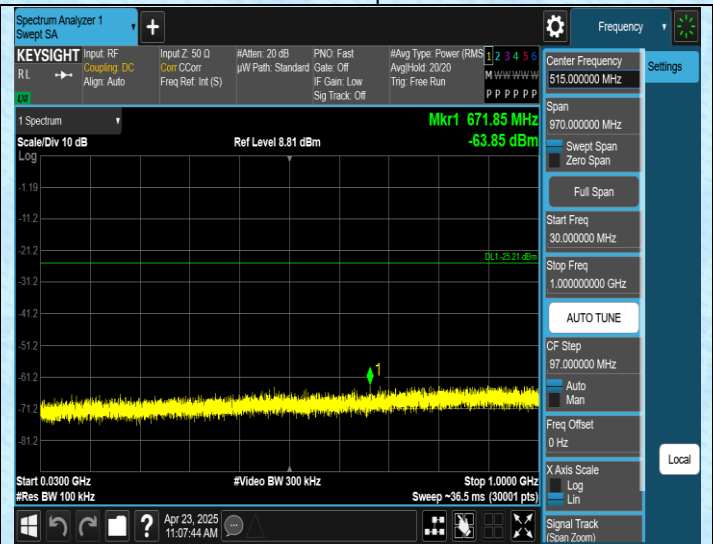
11AX20SISO-Ant1-2462-30~1000-PASS
