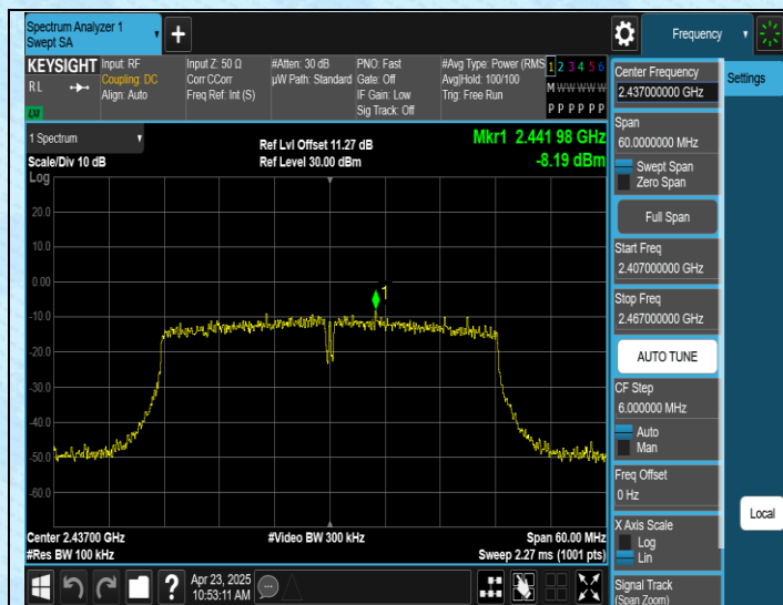
11N40SISO-Ant1-2437-0~Reference-PASS
