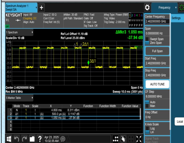
NTNV-11AX20SISO-Ant1-2462
