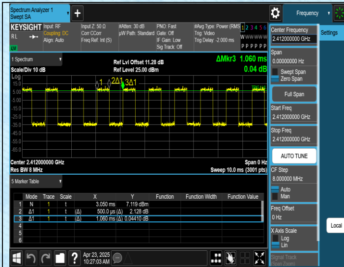
NTNV-11AX20SISO-Ant1-2412
