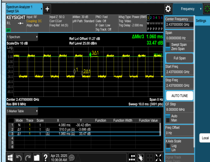
NTNV-11AX40SISO-Ant1-2437
