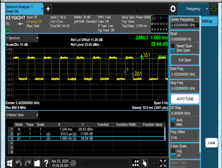
NTNV-11AX40SISO-Ant1-2422
