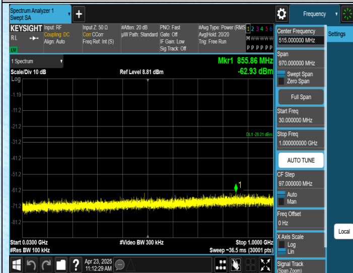
11AX40SISO-Ant1-2452-30~1000-PASS
