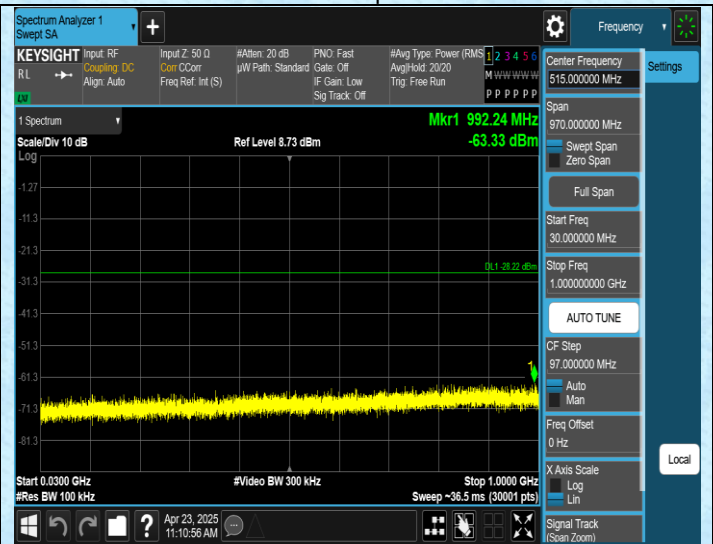
11AX40SISO-Ant1-2437-30~1000-PASS
