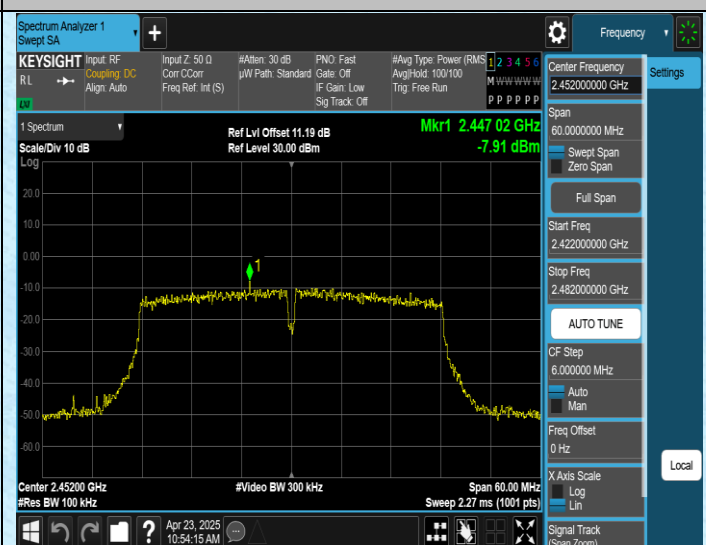
11N40SISO-Ant1-2452-0~Reference-PASS
