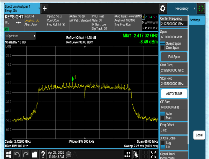
11AX40SISO-Ant1-2422-0~Reference-PASS
