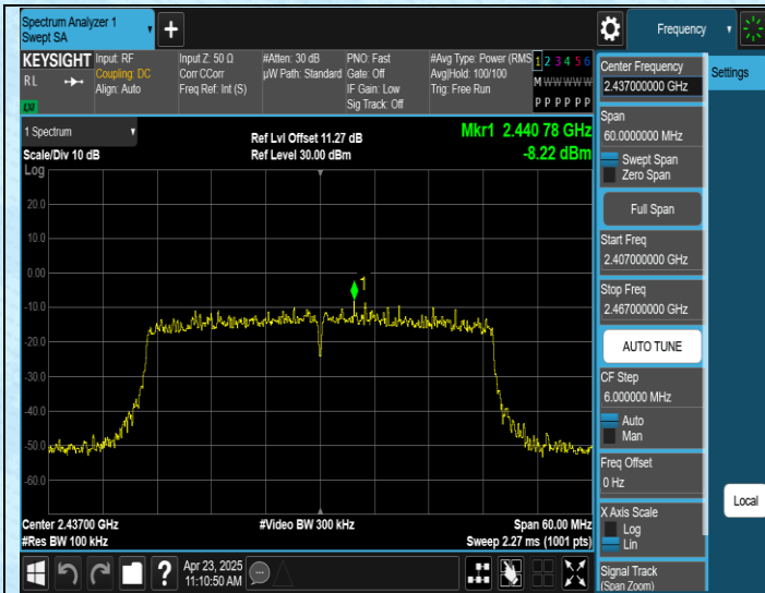
11AX40SISO-Ant1-2437-0~Reference-PASS
