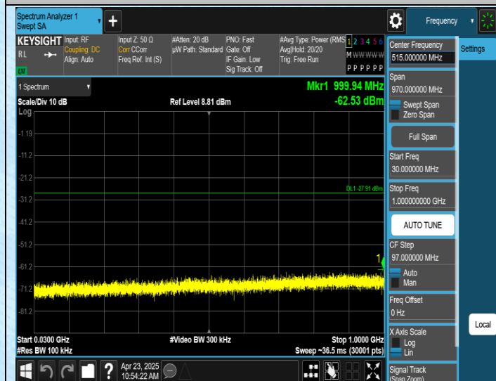
11N40SISO-Ant1-2452-30~1000-PASS
