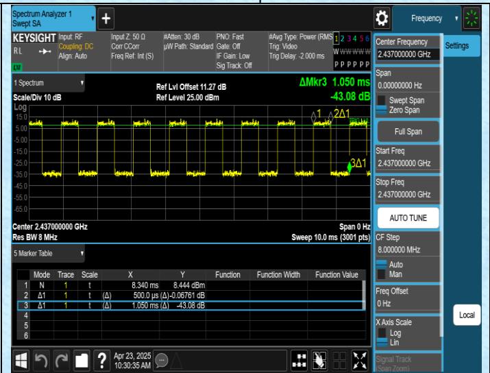
NTNV-11AX20SISO-Ant1-2437
