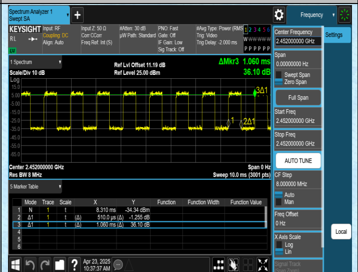
NTNV-11AX40SISO-Ant1-2452
