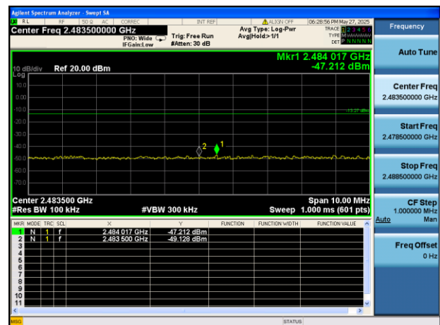
GFSK (1Mbps) HIGH CHANNEL, BAND EDGE
