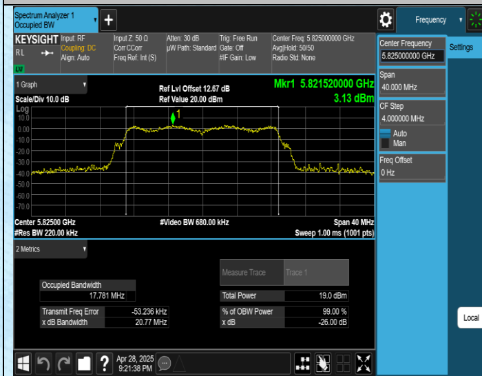
11AC20SISO-Ant1-5825
