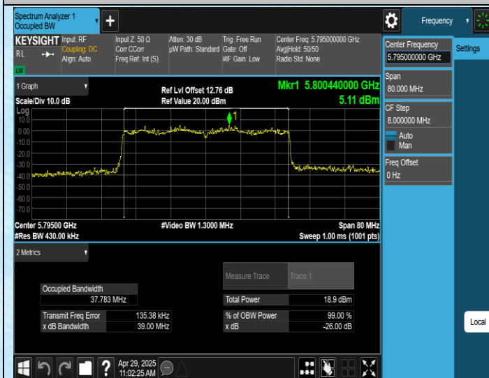
11AX40SISO-Ant1-5795
