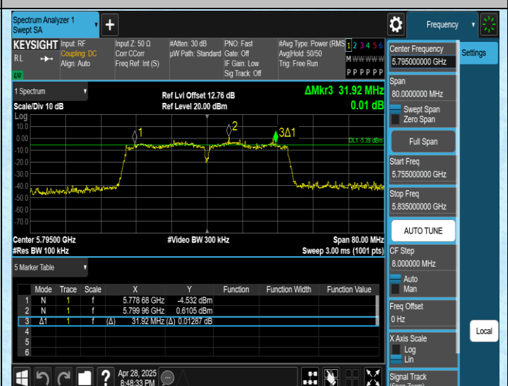
11N40SISO-Ant1-5795-PASS
