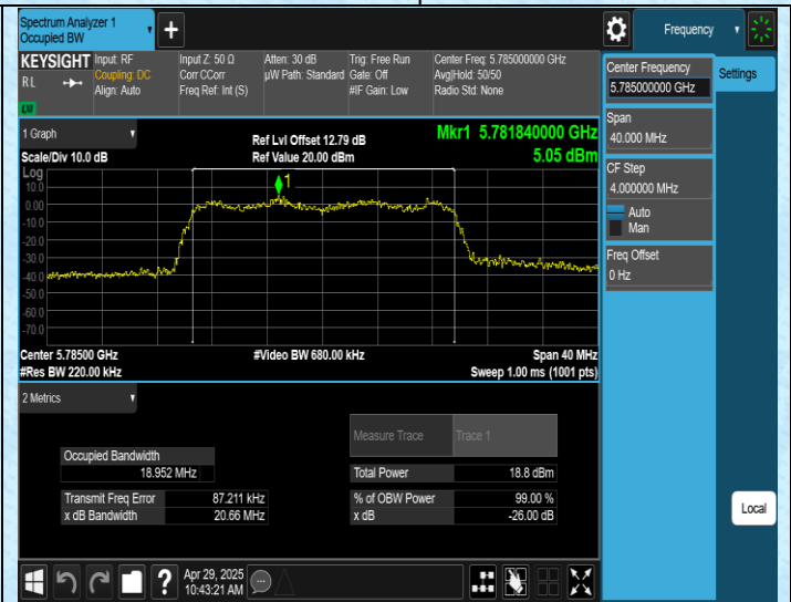
11AX20SISO-Ant1-5785
