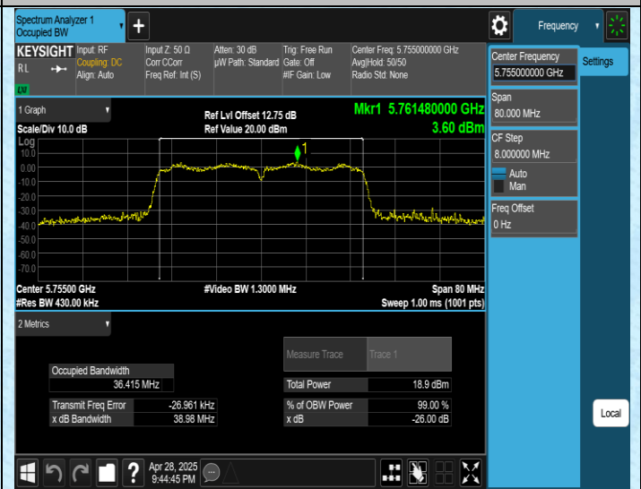
11AC40SISO-Ant1-5755
