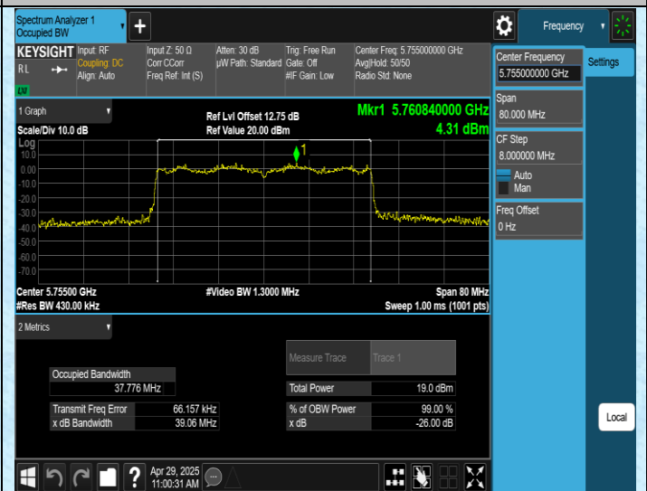
11AX40SISO-Ant1-5755
