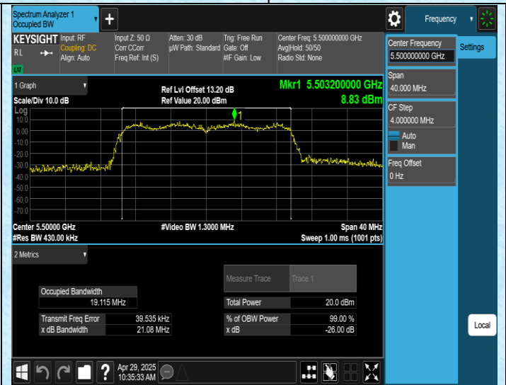
11AX20SISO-Ant1-5500
