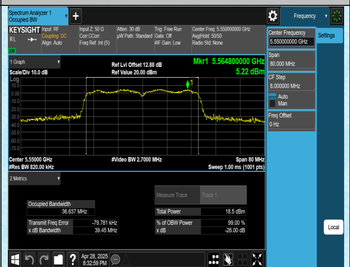
11N40SISO-Ant1-5550
