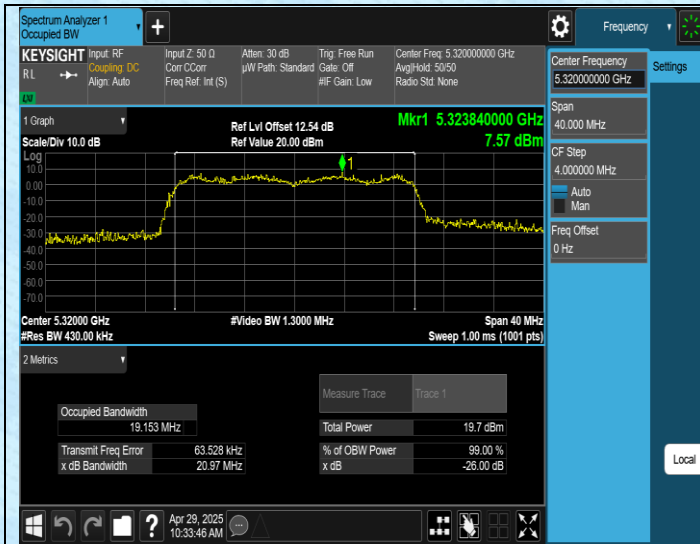
11AX20SISO-Ant1-5320
