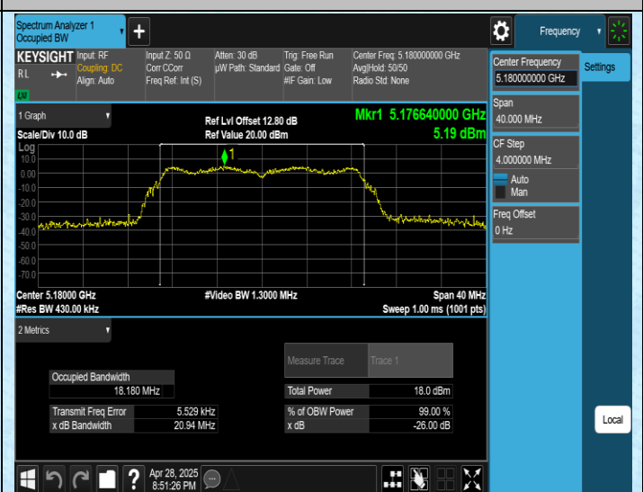
11AC20SISO-Ant1-5180
