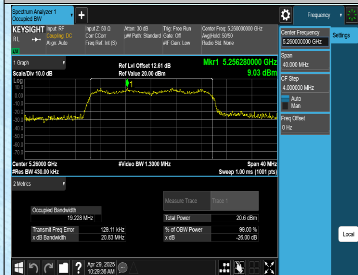
11AX20SISO-Ant1-5260
