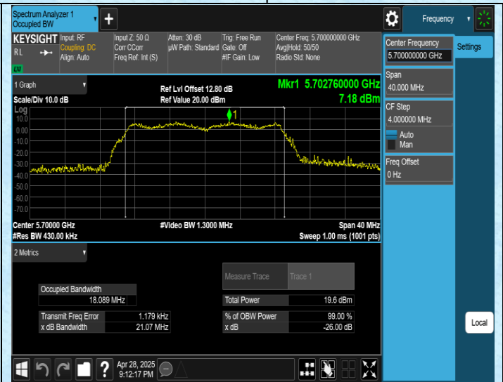
11AC20SISO-Ant1-5700
