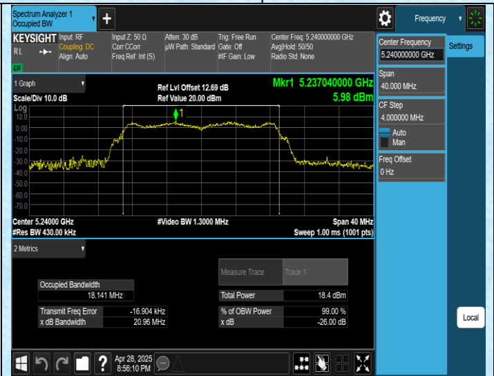
11AC20SISO-Ant1-5240
