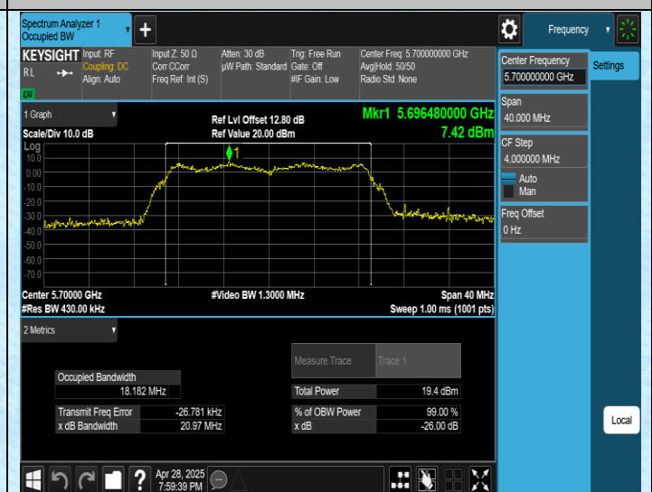
11N20SISO-Ant1-5700
