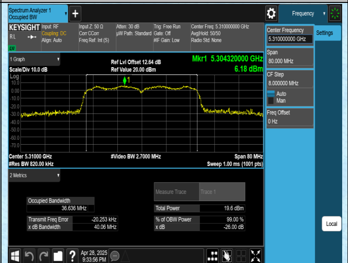
11AC40SISO-Ant1-5310
