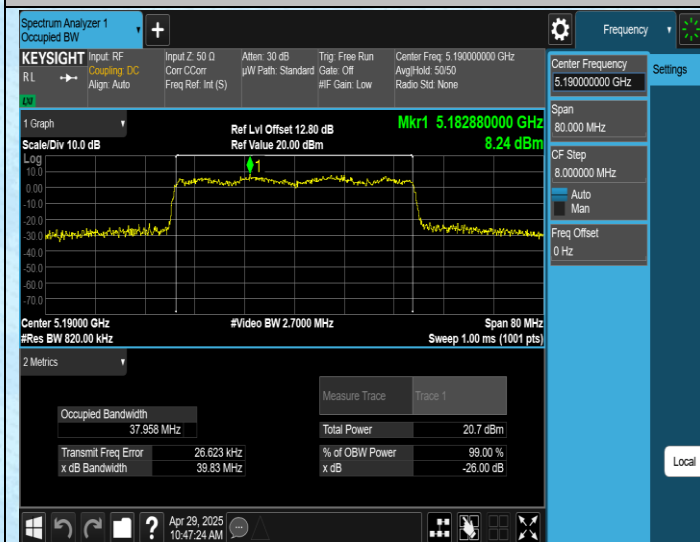
11AX40SISO-Ant1-5190
