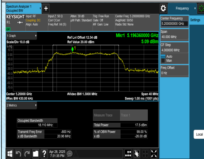
11N20SISO-Ant1-5200
