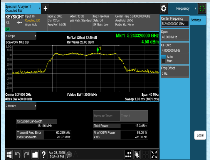
11N20SISO-Ant1-5240
