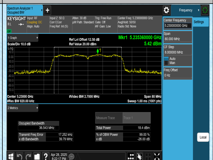
11N40SISO-Ant1-5230
