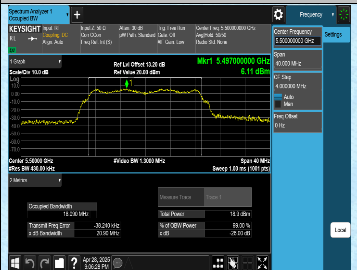
11AC20SISO-Ant1-5500
