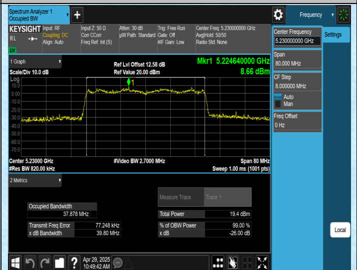
11AX40SISO-Ant1-5230
