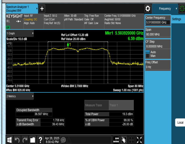
11N40SISO-Ant1-5510
