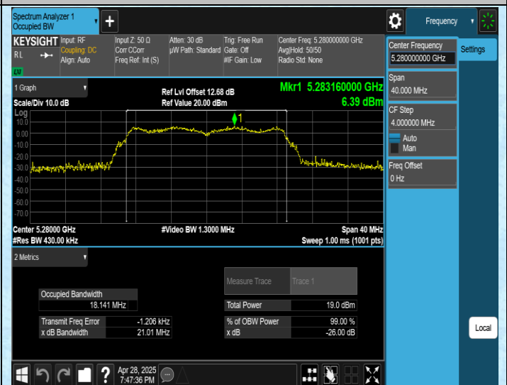
11N20SISO-Ant1-5280
