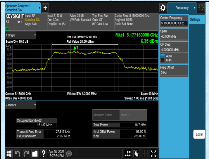
11N20SISO-Ant1-5180
