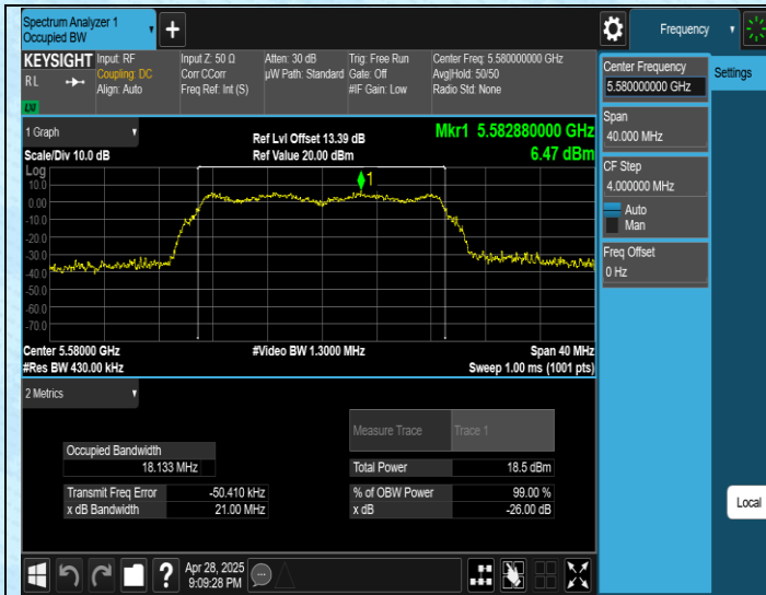
11AC20SISO-Ant1-5580
