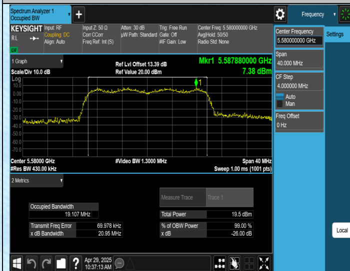
11AX20SISO-Ant1-5580
