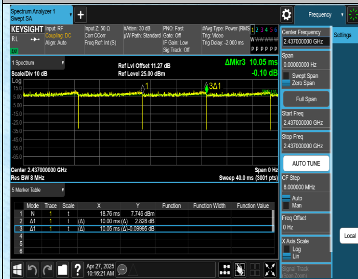
NTNV-11N40SISO-Ant1-2437
