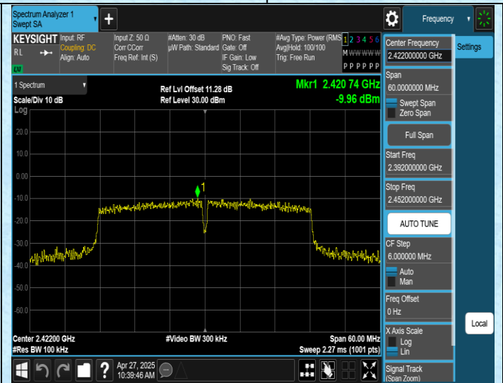
11N40SISO-Ant1-2422-0~Reference-PASS
