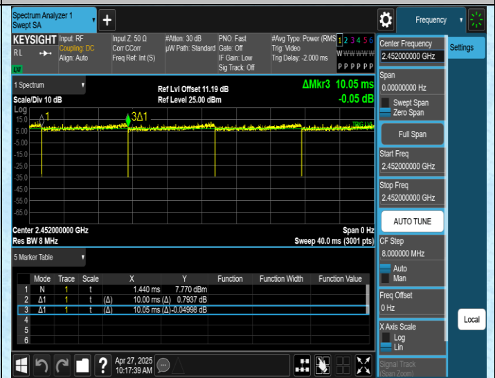
NTNV-11N40SISO-Ant1-2452
